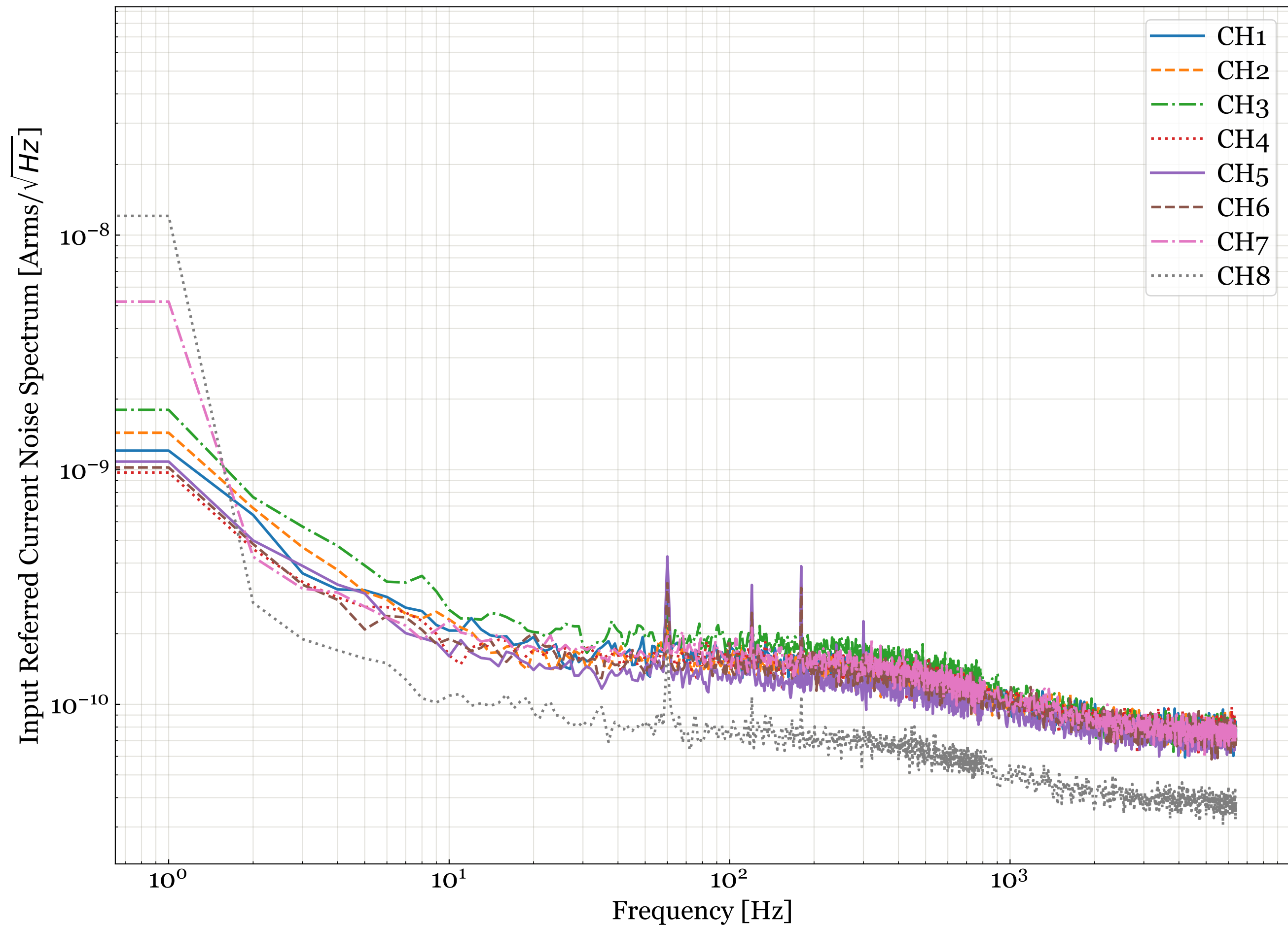
D11000687 S2100029 Input Referred Current Noise Spectrum.
