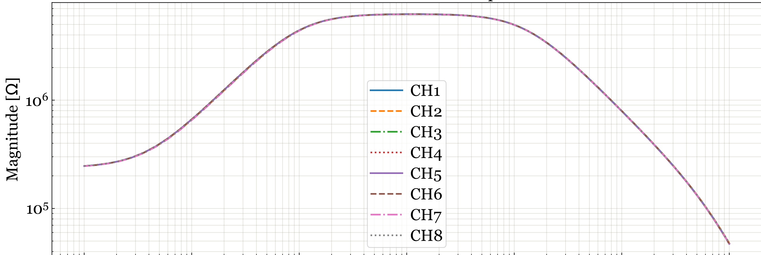
D11000687 S2100029 Transimpedance Transfer Function. Series resistance of 12kOhm added at input to measure.
