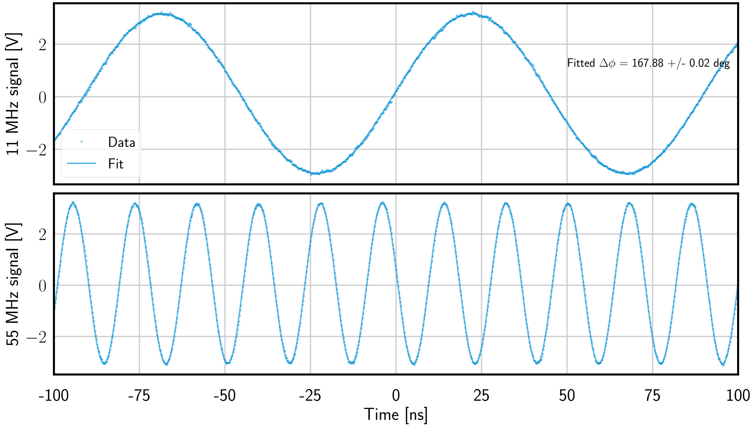
Relative phasing between 11 MHz and 55 MHz signals (EOM path), post-Modification
