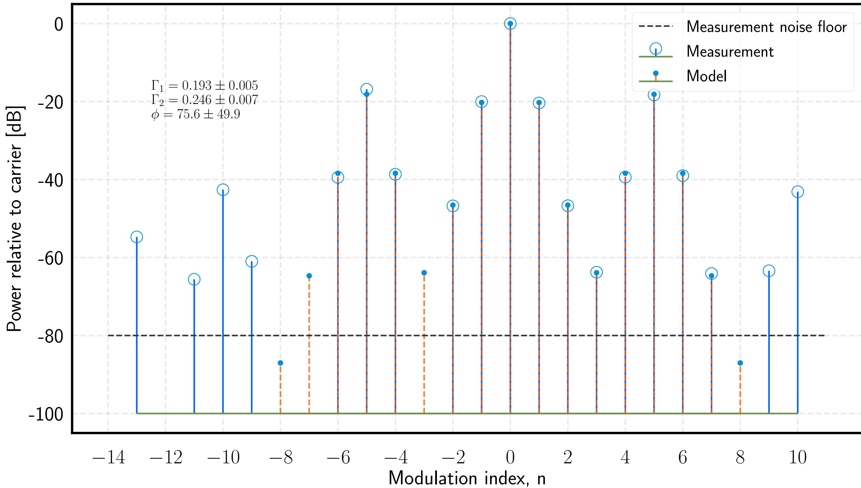
40m PSL beam RF modulation spectrum, Dec 2020
