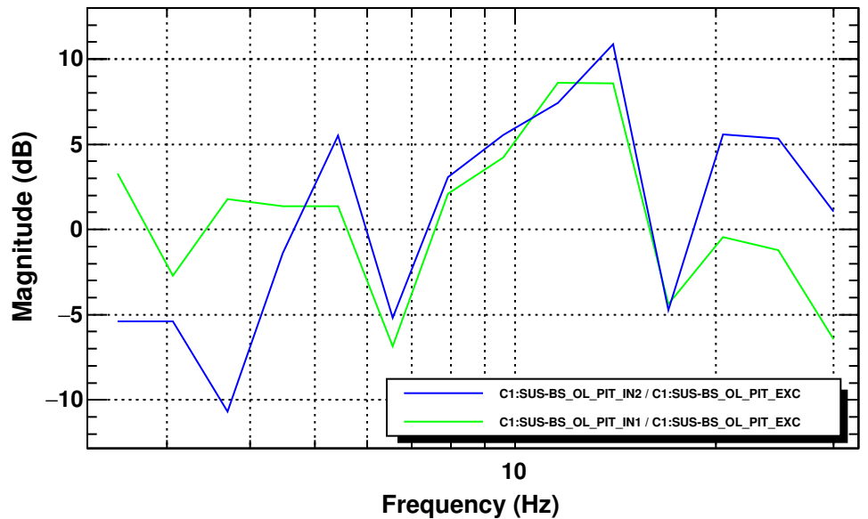
Transfer function
