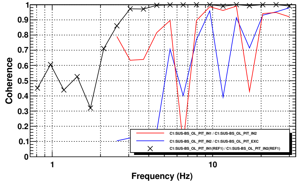
Coherence function
