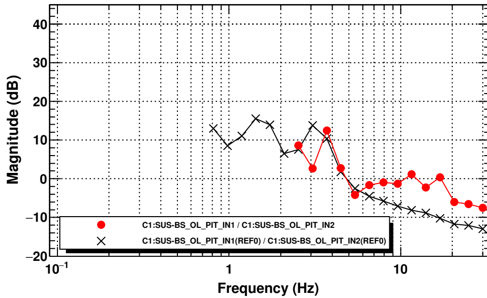
Open Loop Gain
