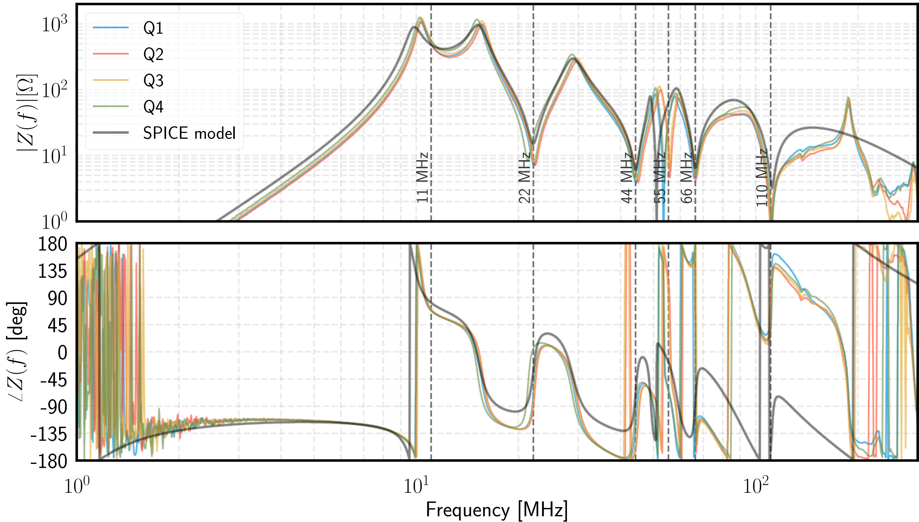
RF Low path transimpedance measurement
