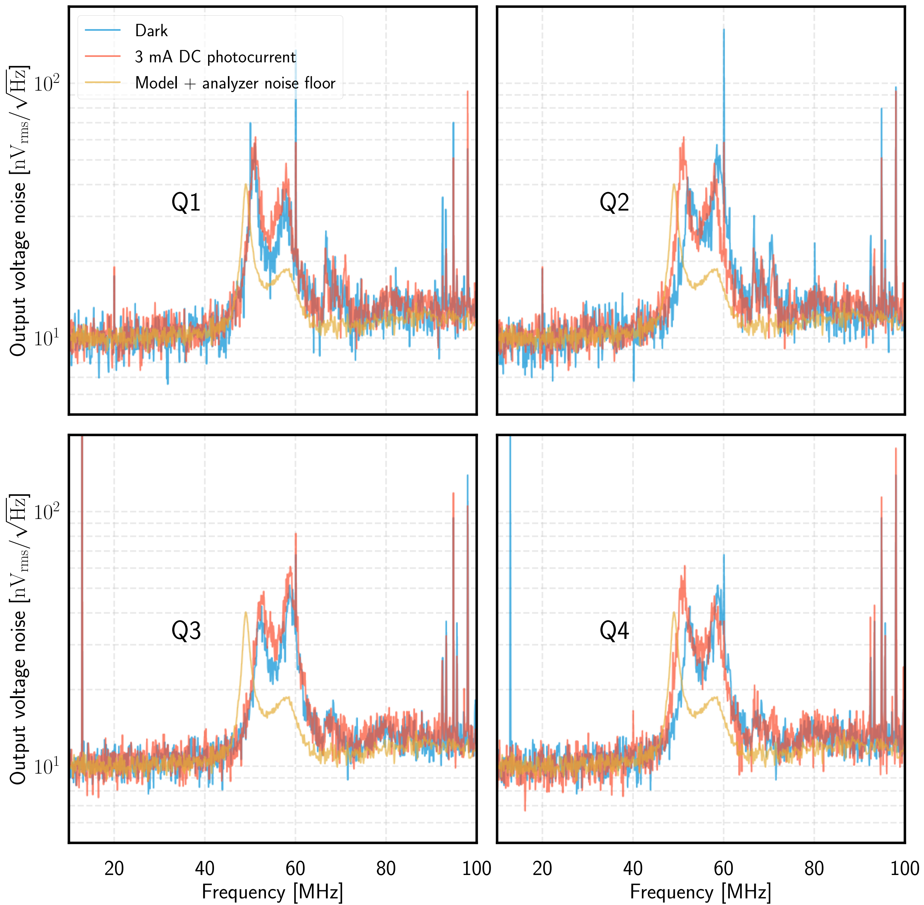
Voltage noise of WFS quadrants
