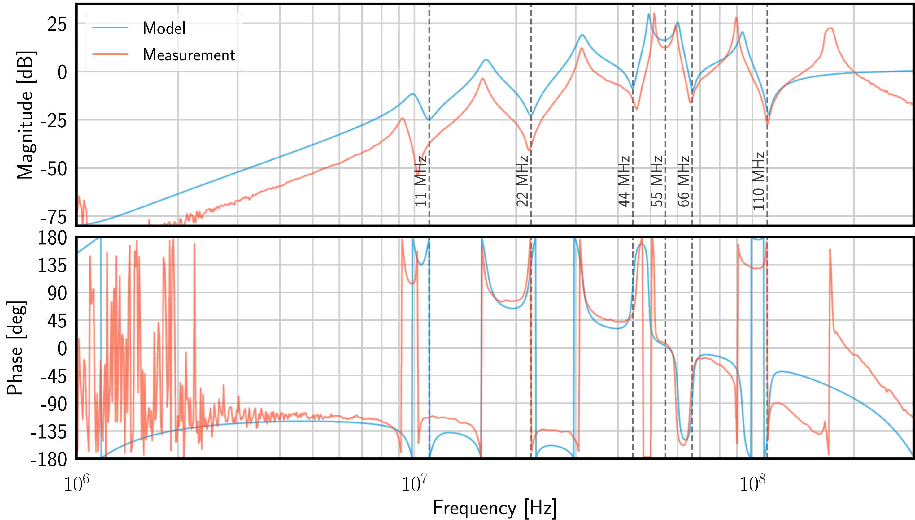
Model vs measurement of TF from current injection path to RF High output for 40m WFS head circuit
