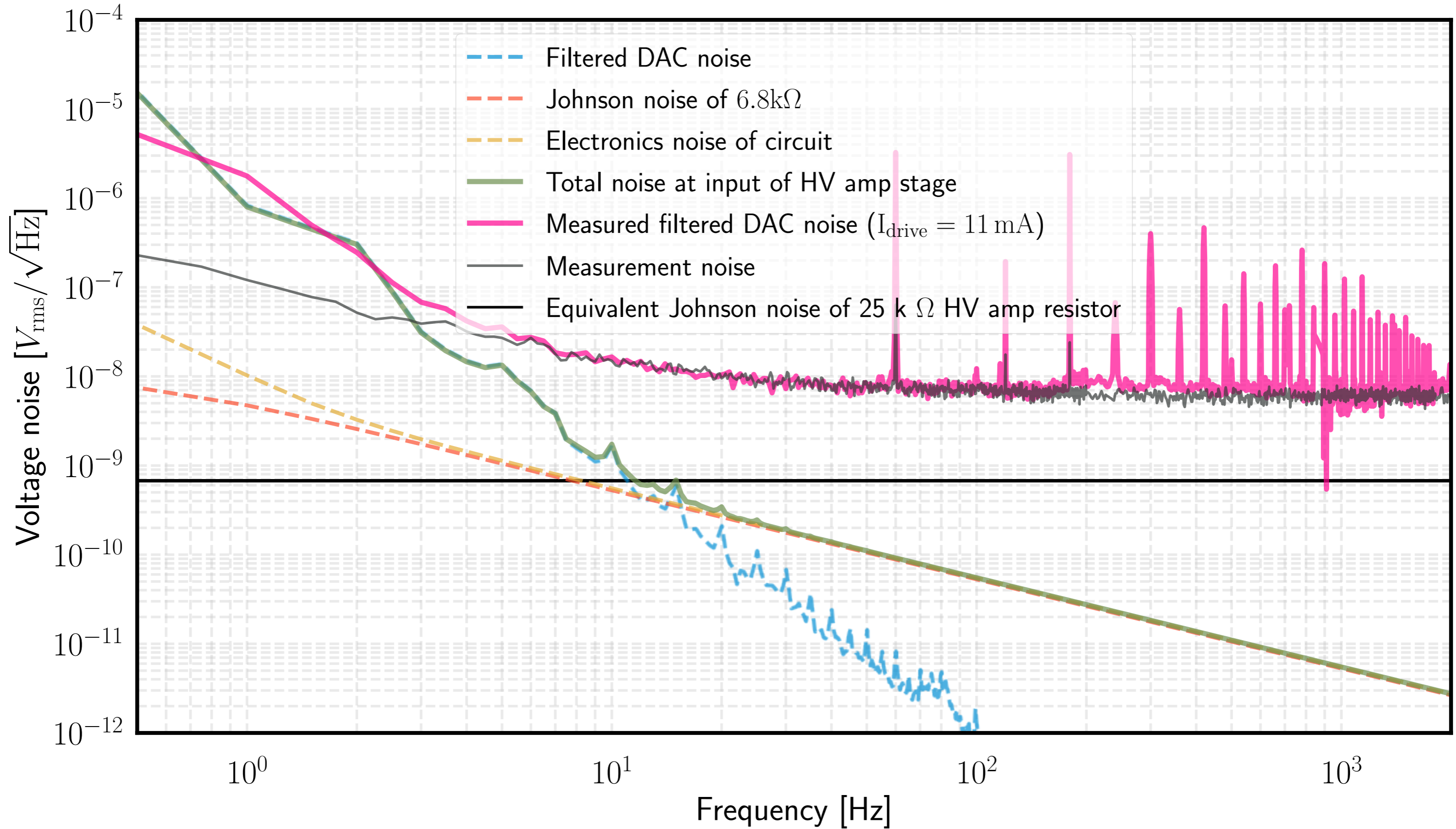
Noise contributions from DAC noise filtering stage
