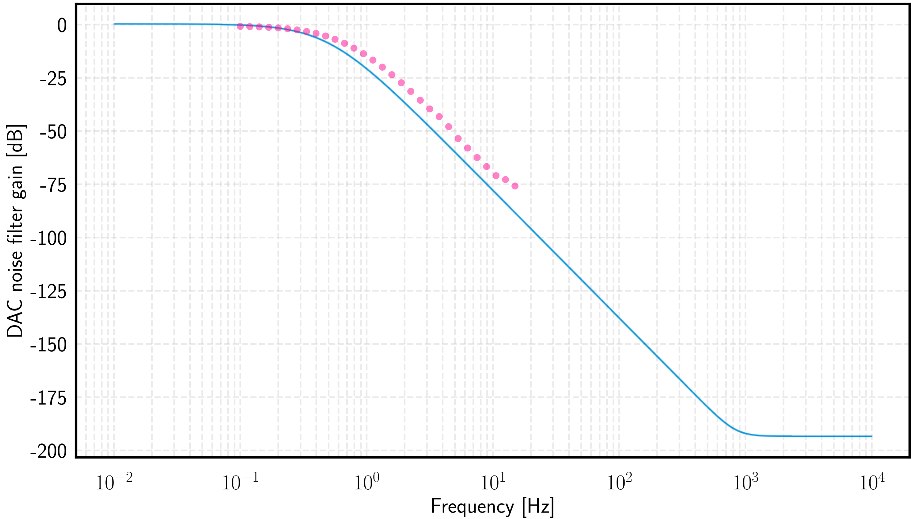
DAC noise filter gain
