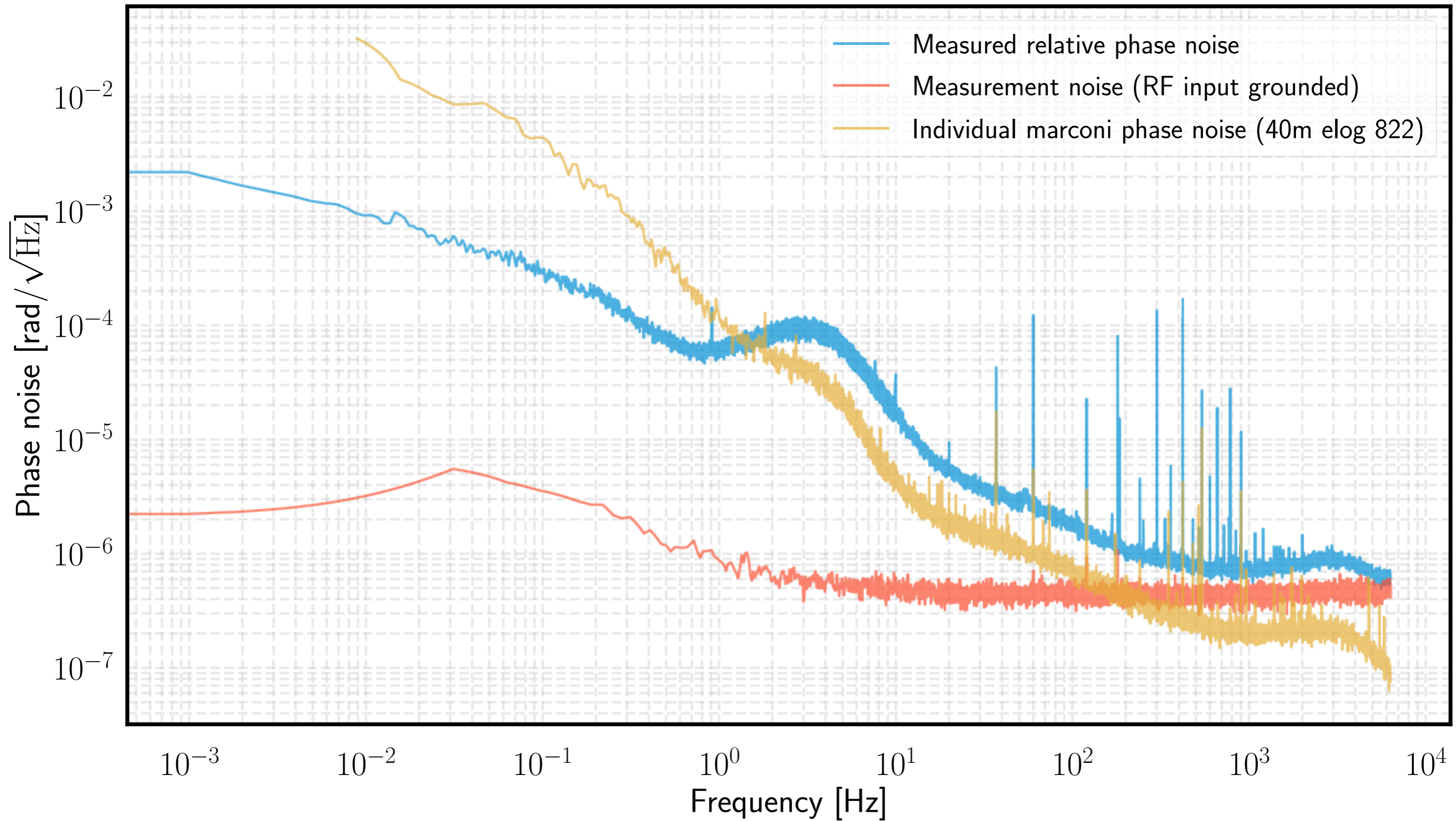
Relative stability of two marconis synchronized to FS725 Rb standard
