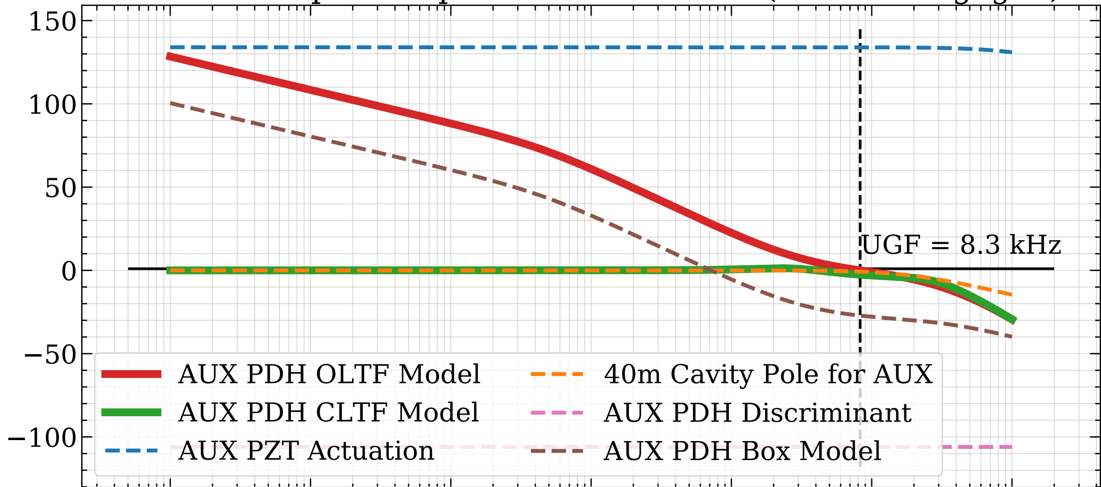
AUX PDH Open Loop Transfer Function (ALS not engaged)
