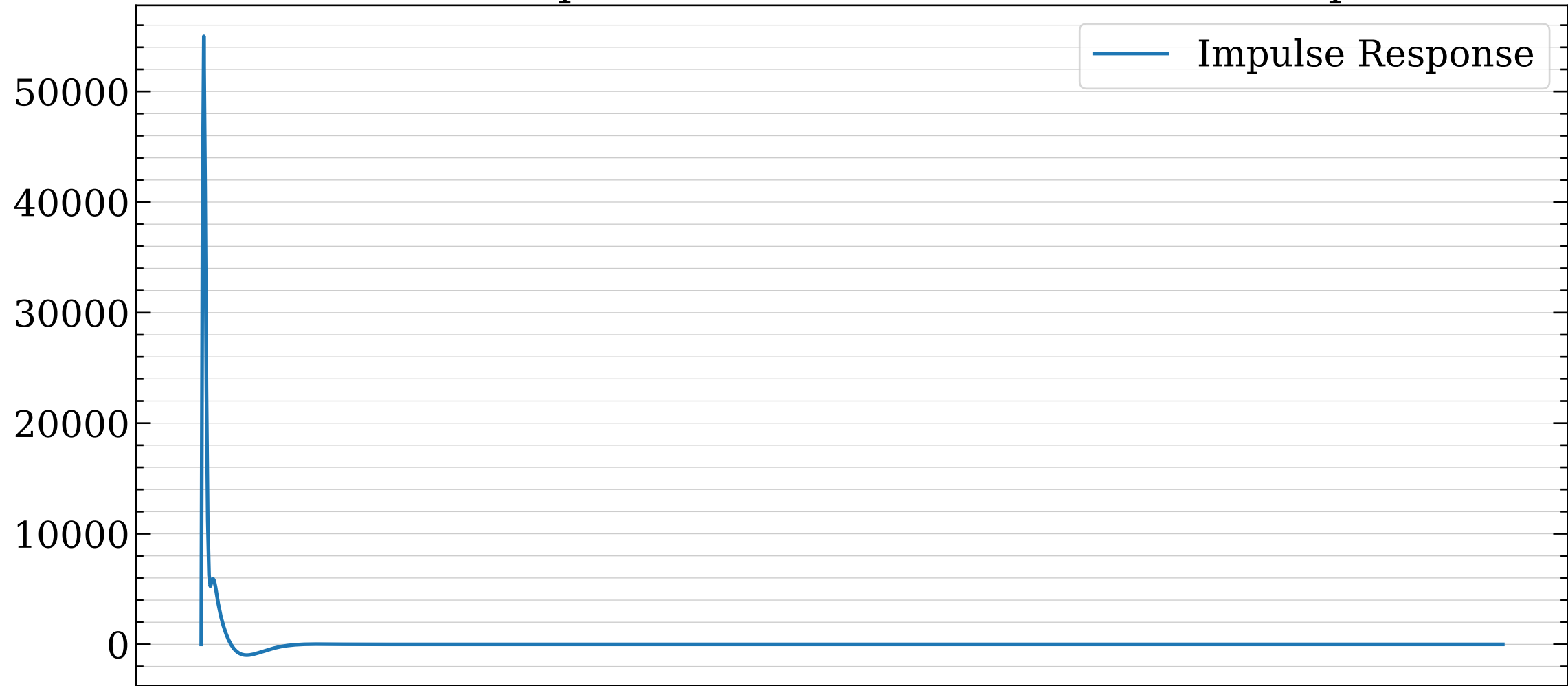
AUX PDH Loop Control Model Time Domain Response
