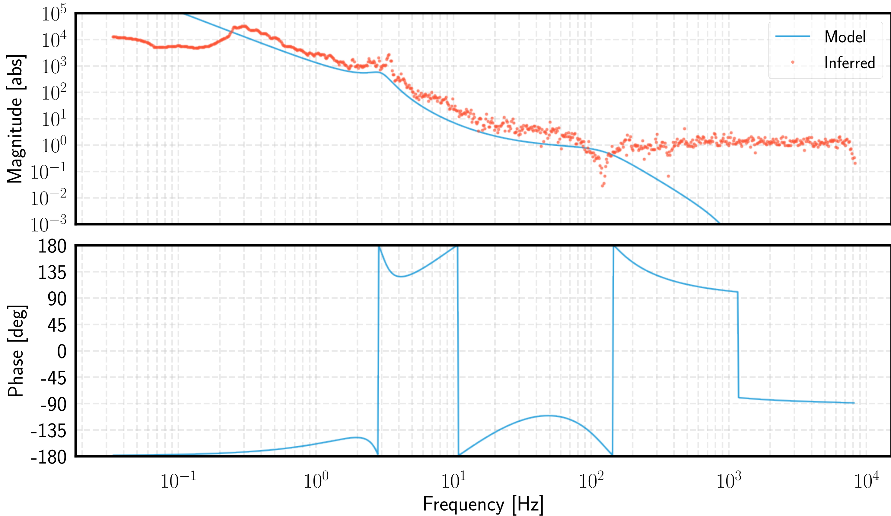
Modelled OLG of digital feedback loop
