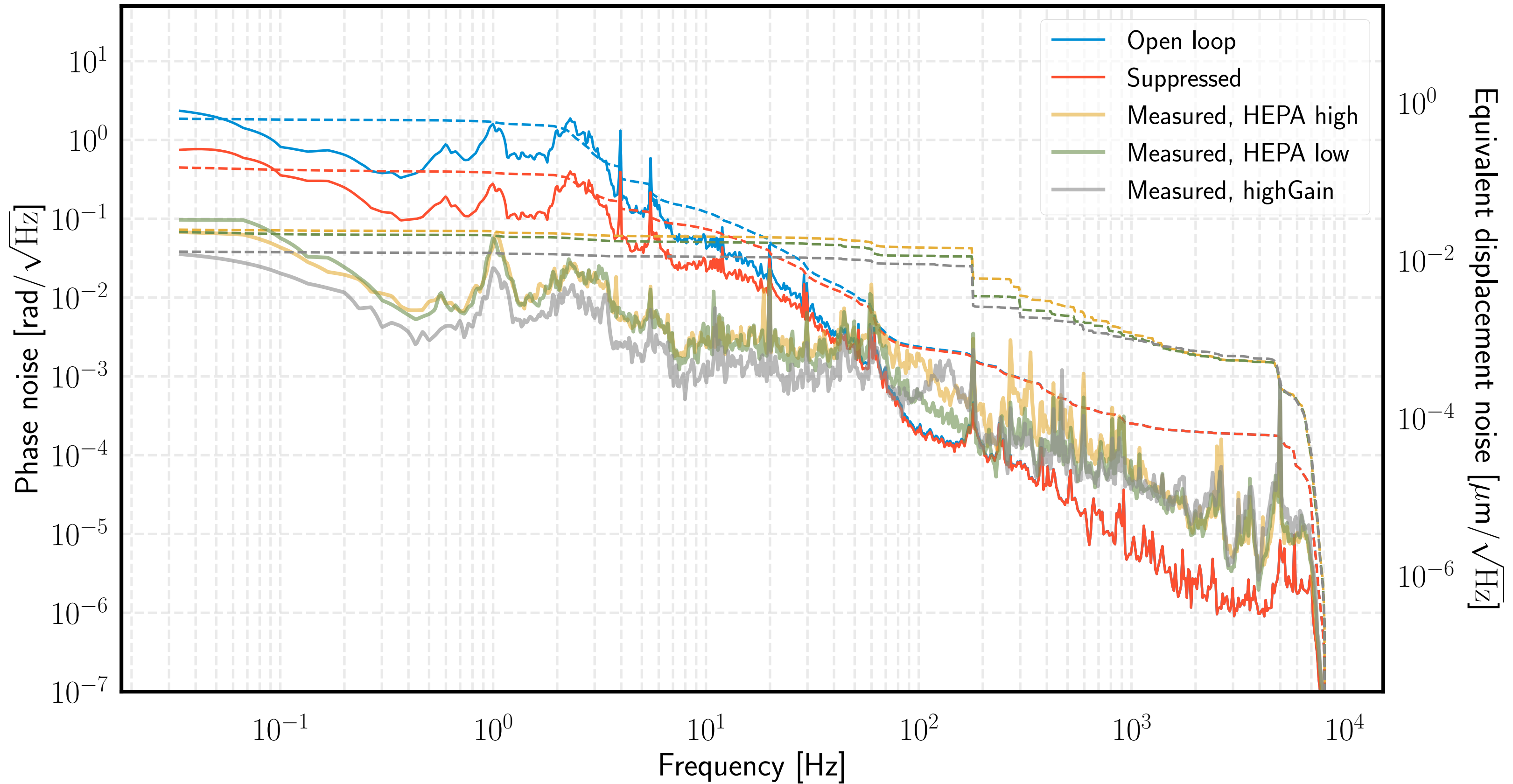
Projected and measured suppression of error signal
