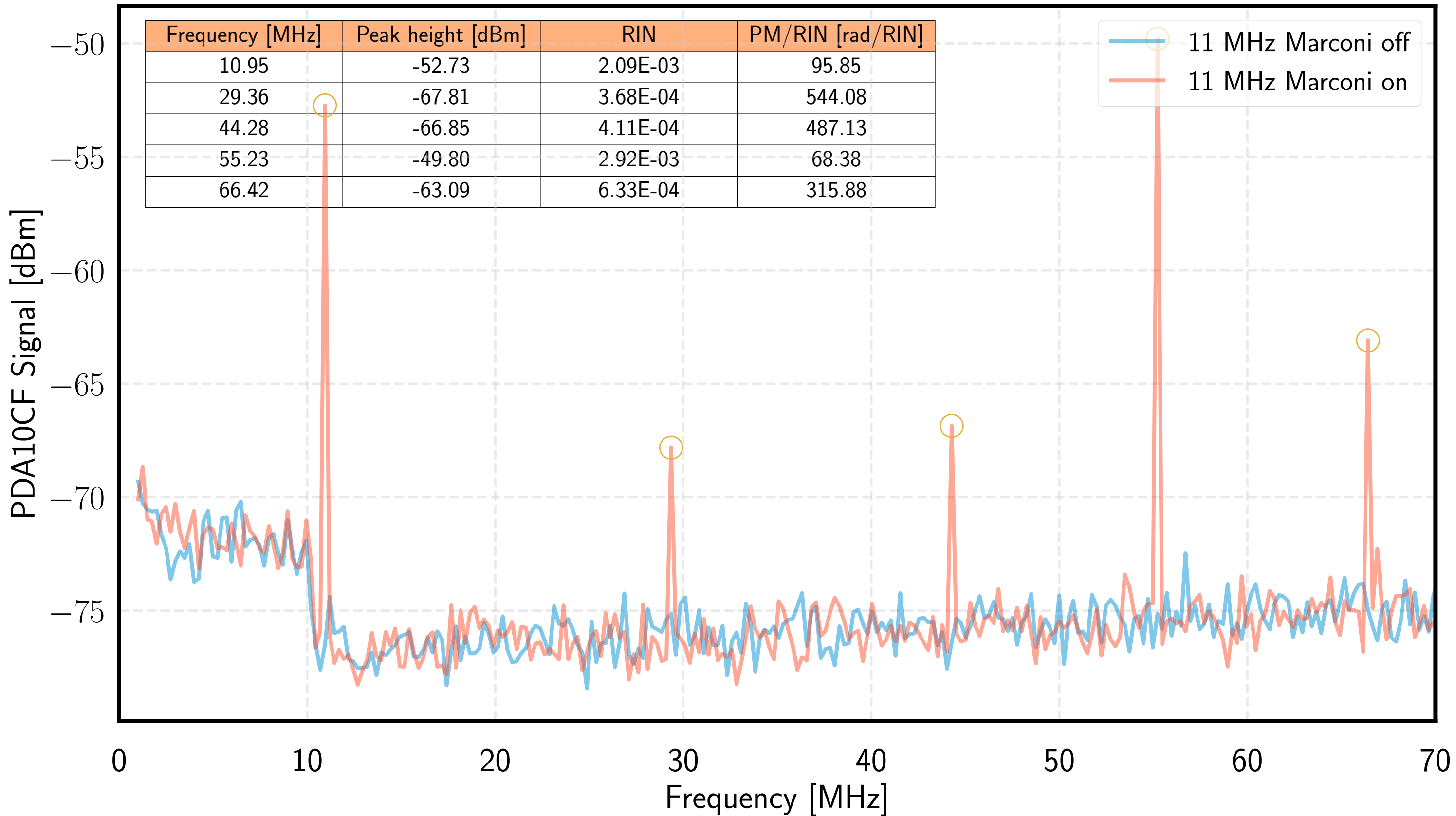
Estimation of RIN and RAM in BHD LO beam
