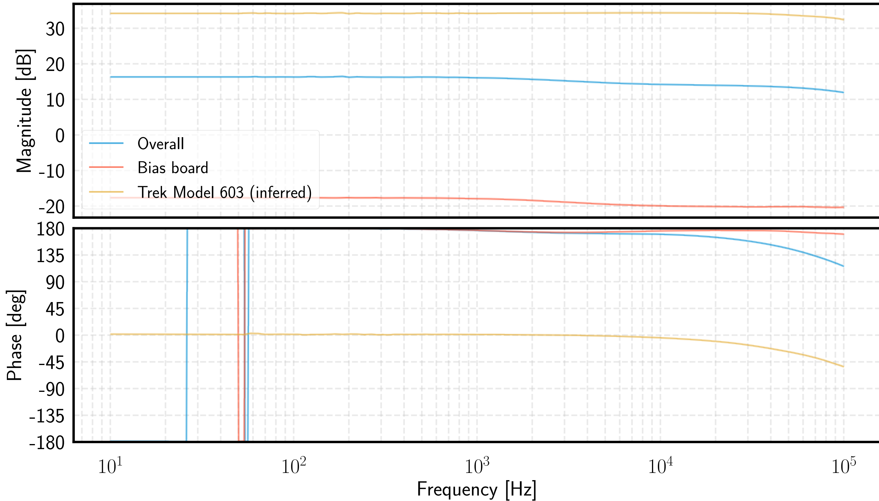
Trek high voltage amplifier TF measurement
