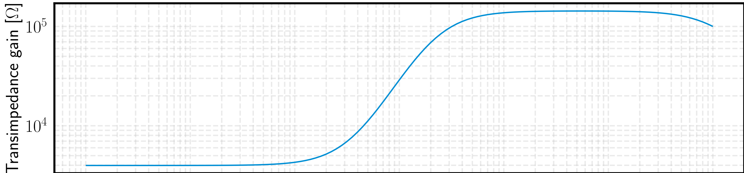
40m DCPD amplifier gain and noise
