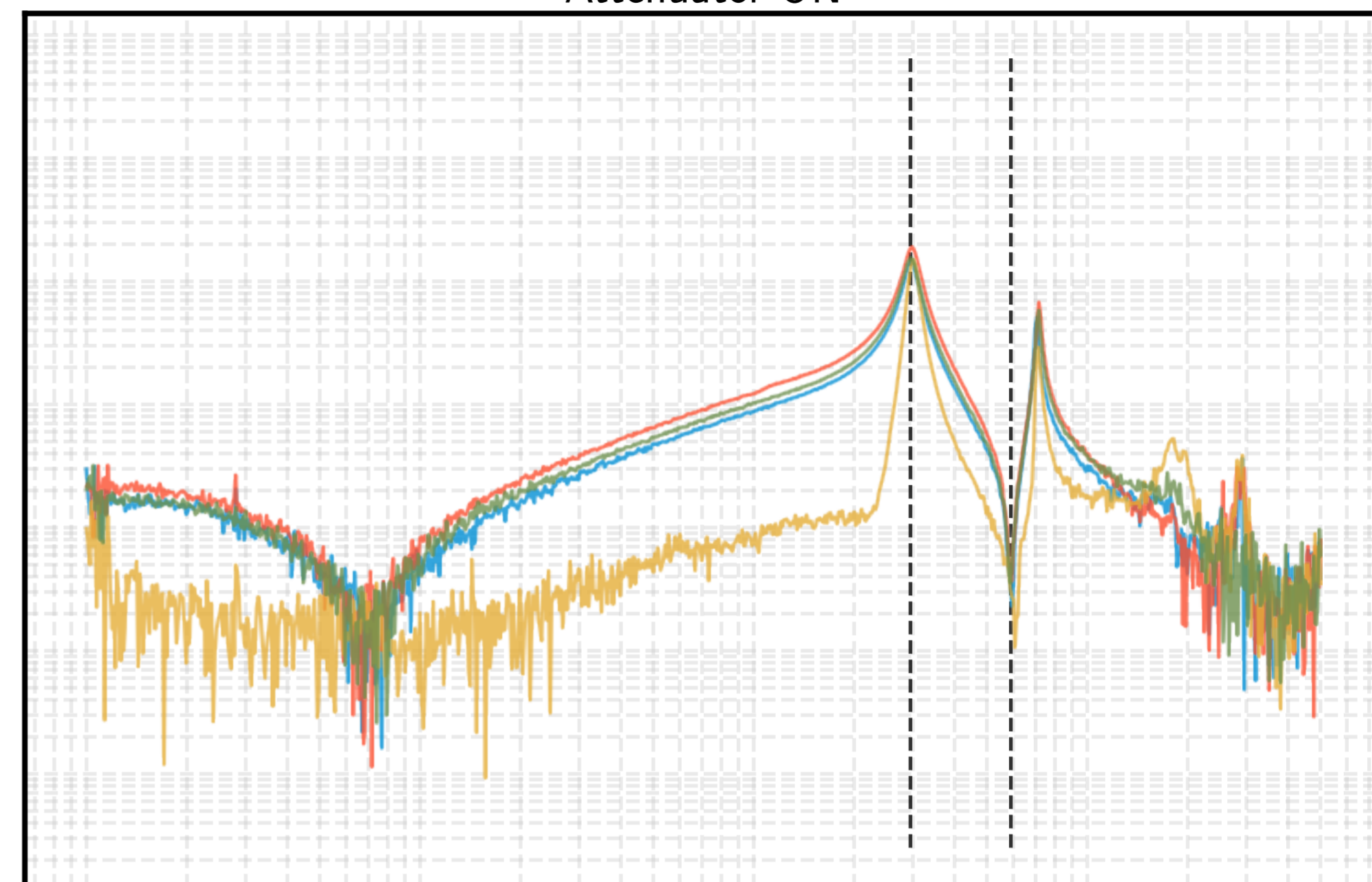
Attenuator ON
