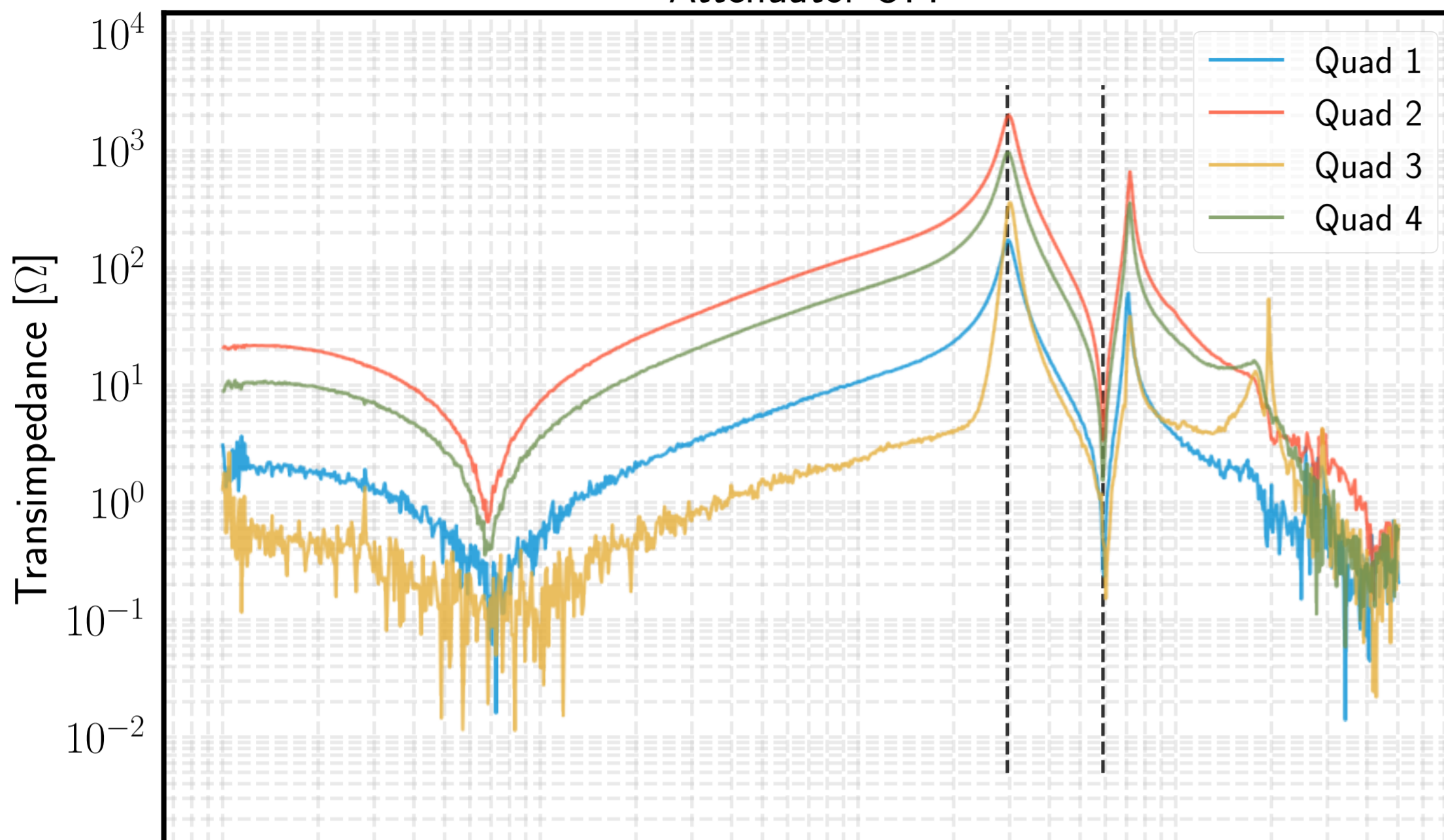
Attenuator OFF
