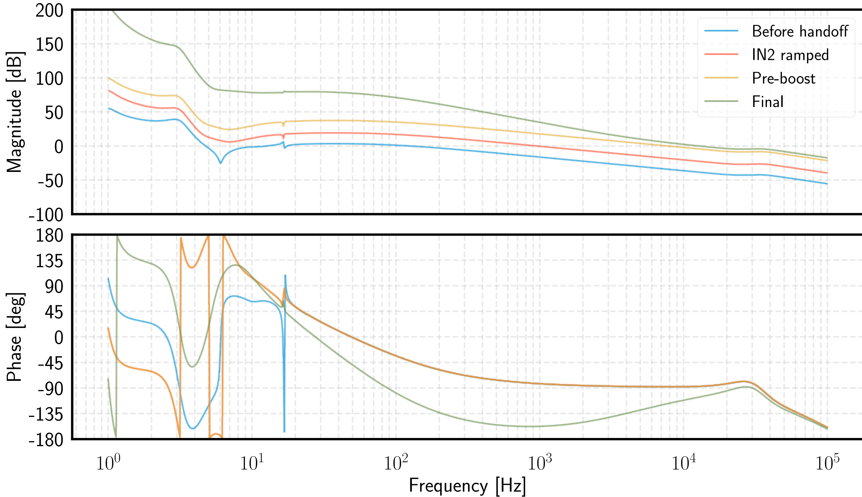
CARM OLG evolution during lock acquisition
