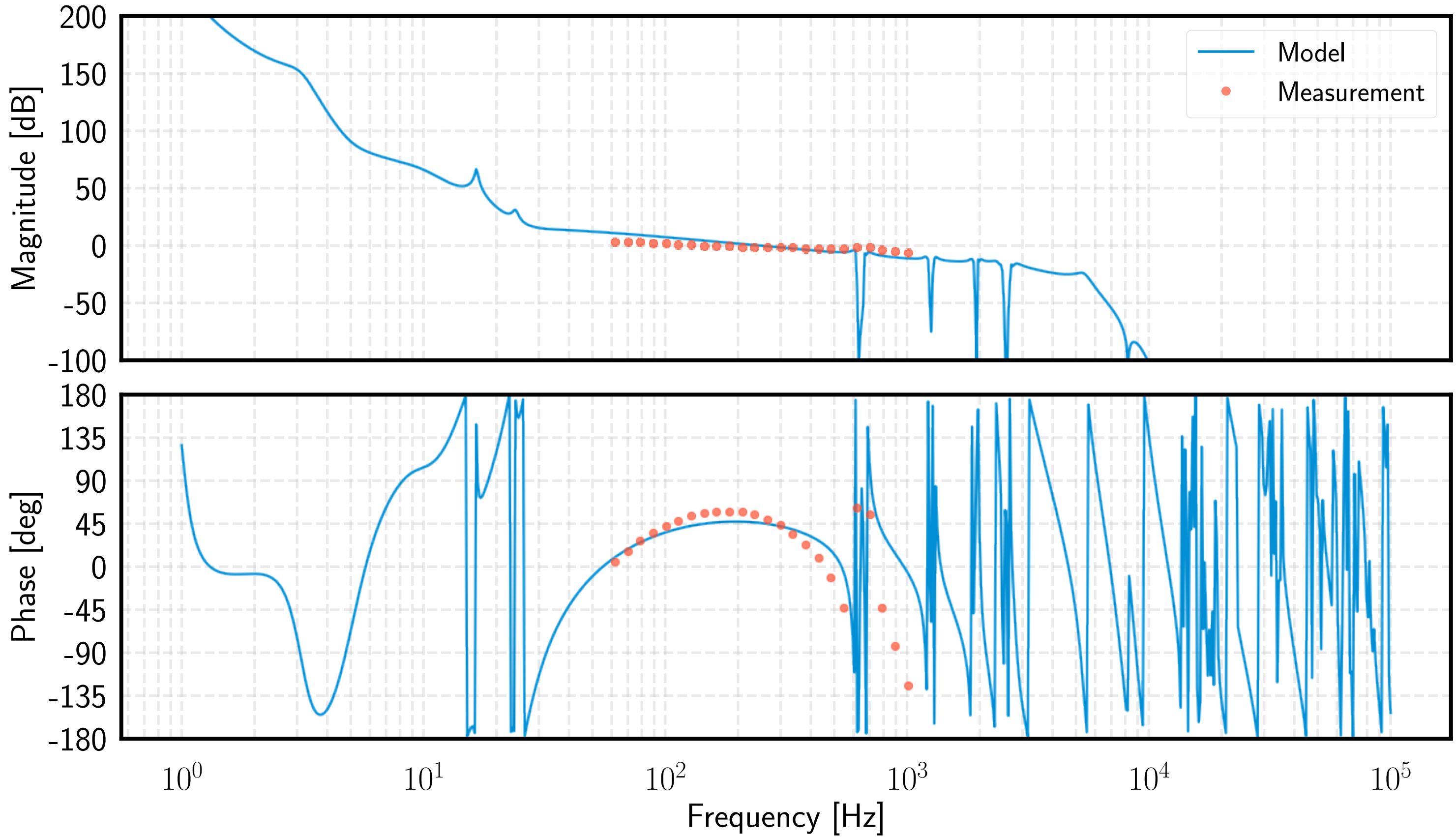
CARM crossover model and measurement
