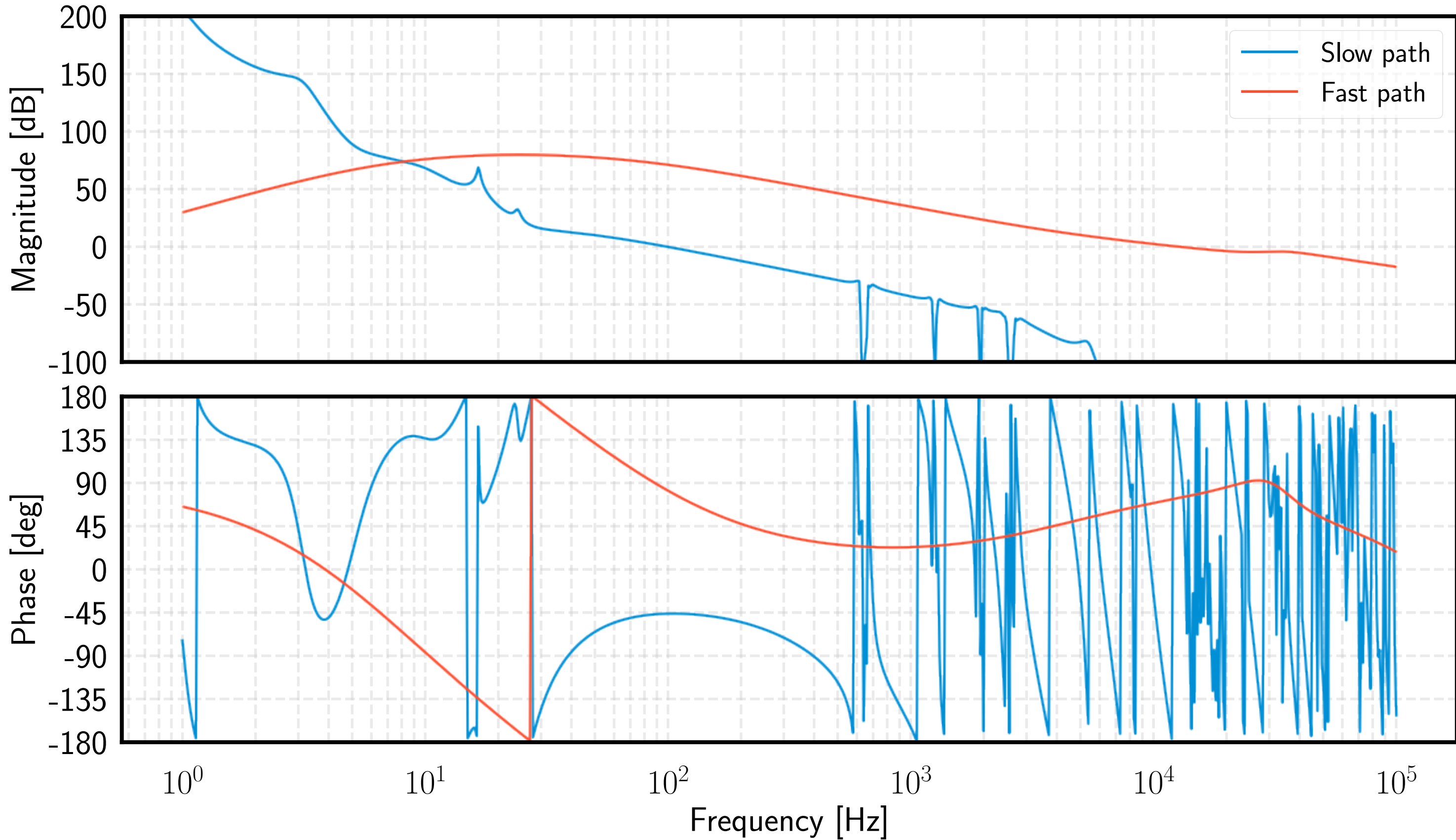
CARM TFs - CM Slow path and AO path
