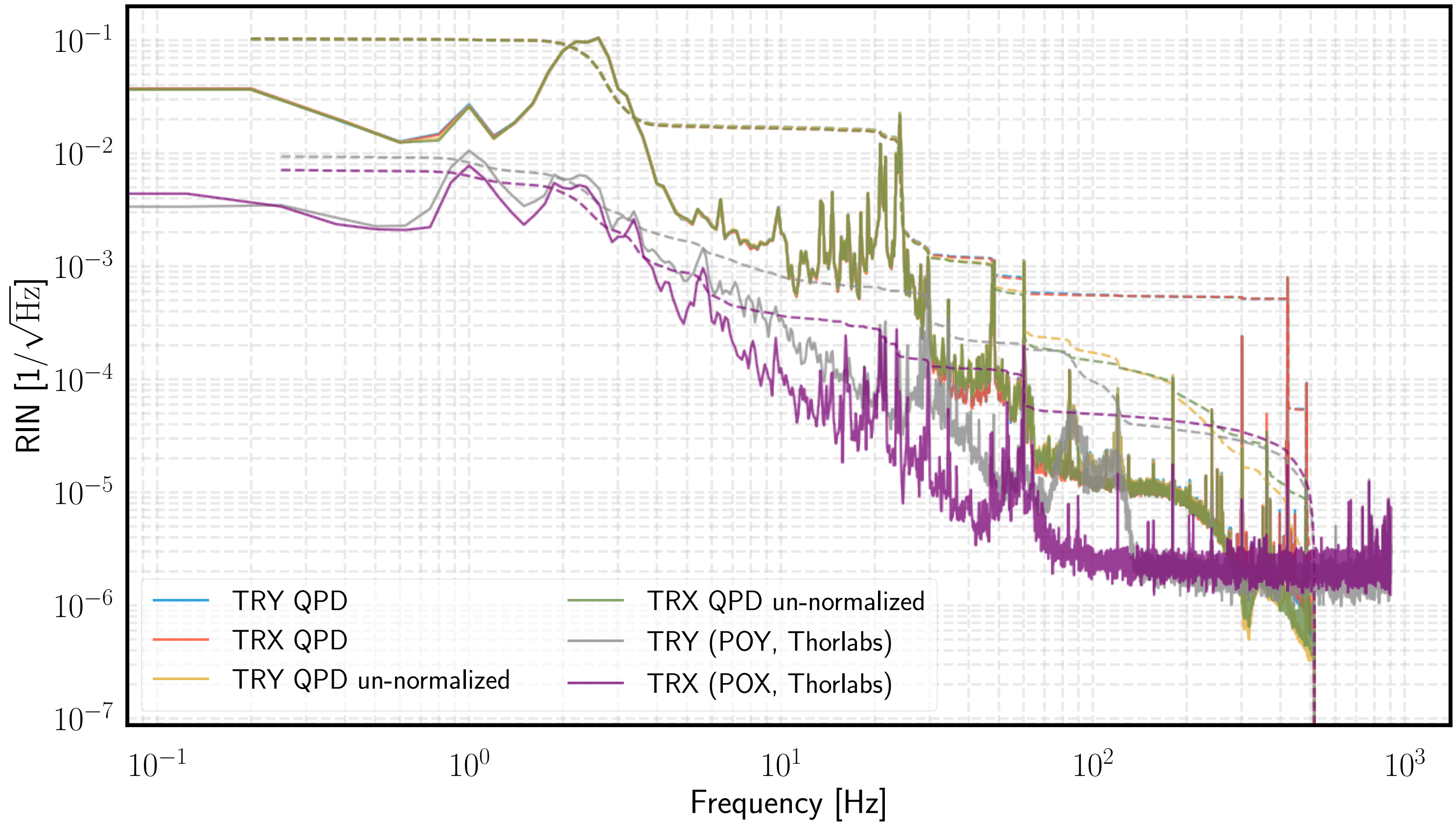
Arm transmission RIN for single arm lock vs PRFPMI
