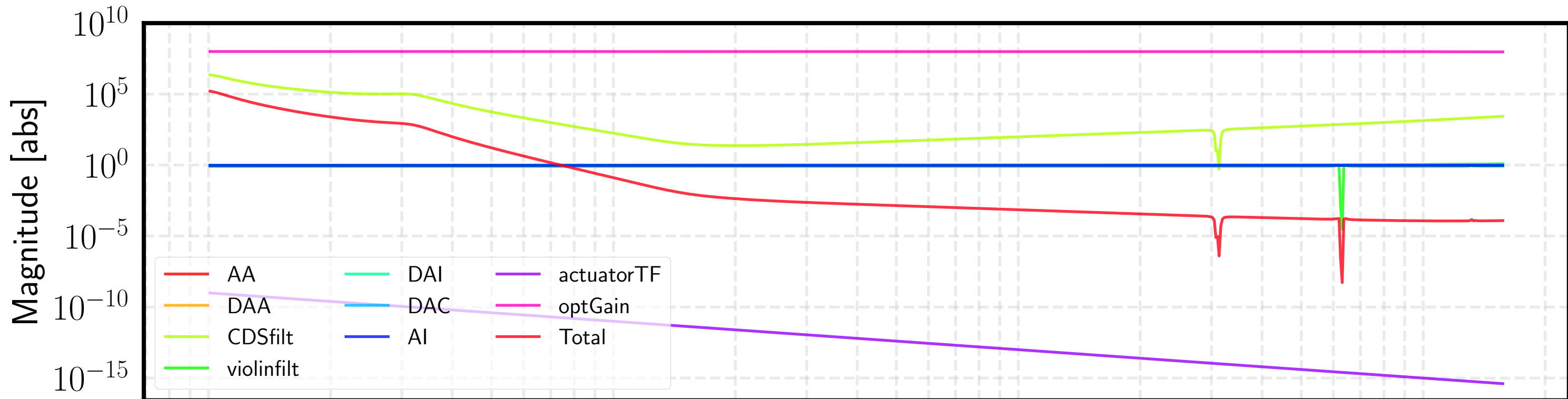
PRFPMI DARM loop model components
