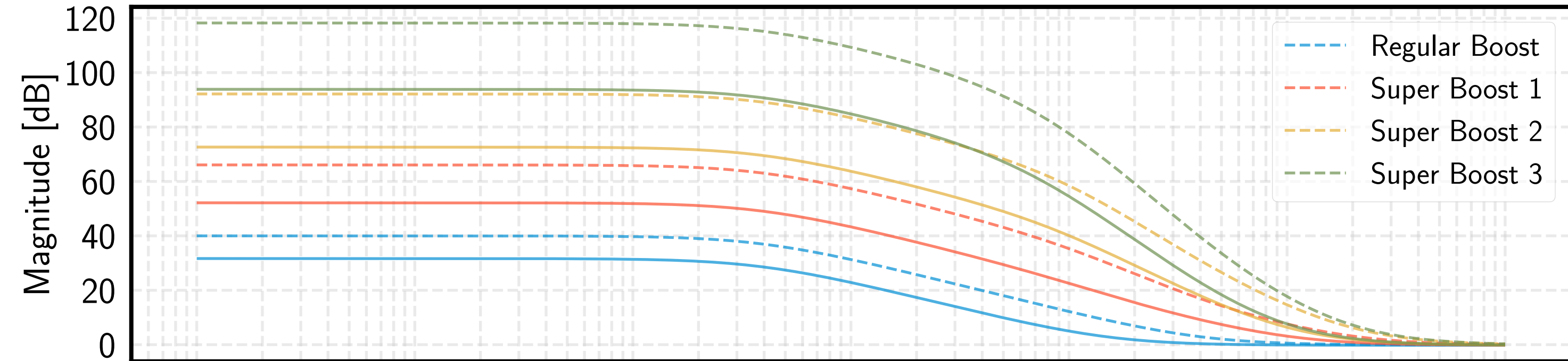
40m CM Board boosts (solid lines are proposed, dashed are as built)
