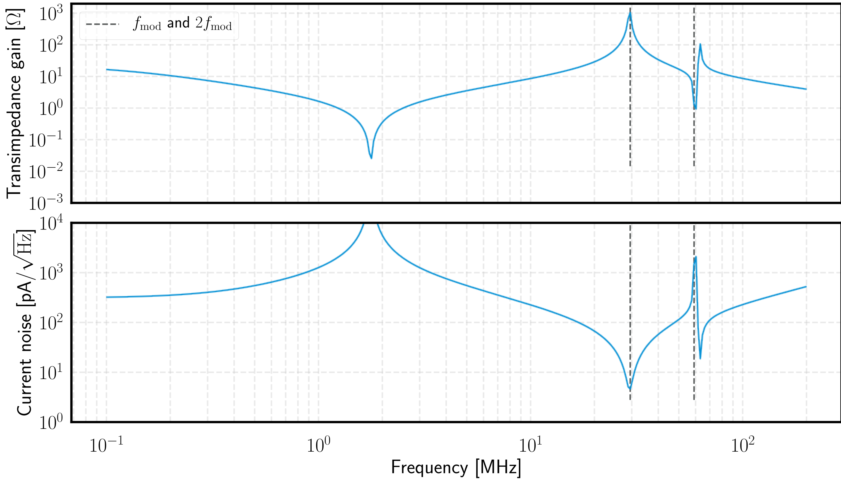
40m IMC WFS head transimpedance gain and noise
