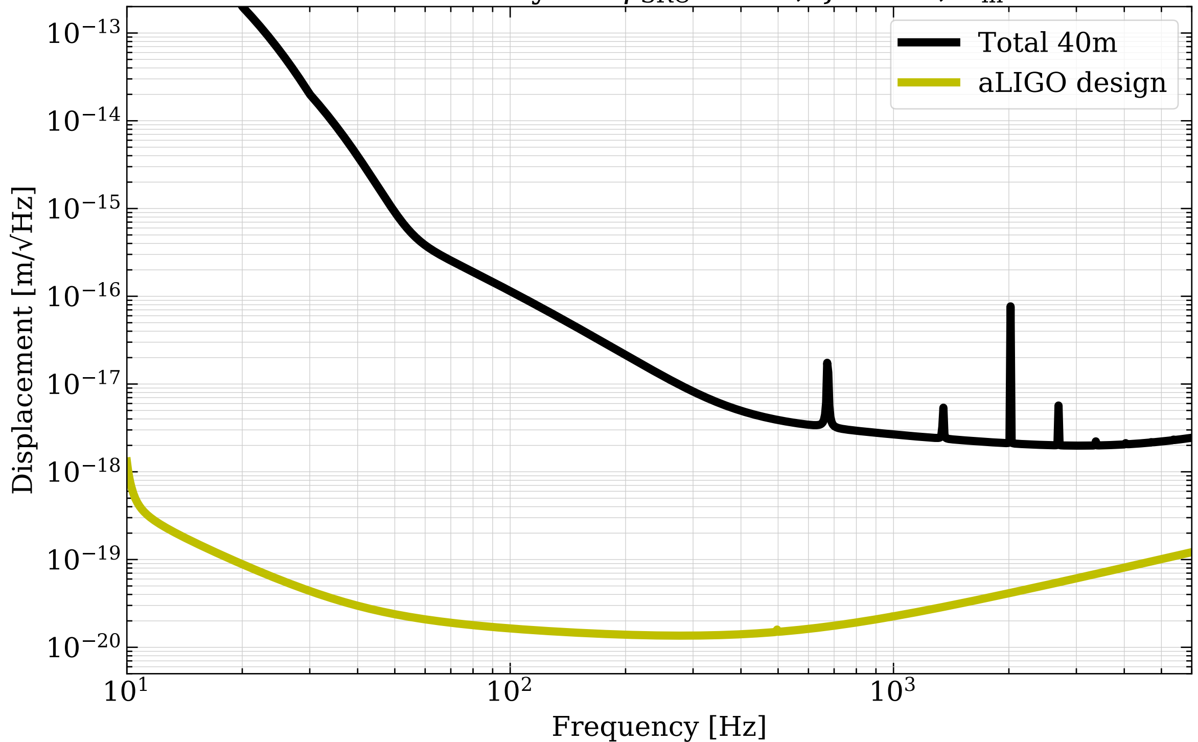
40m DARM sensitivity for \phi_{\text{SRC}} = 0.0^\circ , \zeta = 0.0^\circ , P_{\text{in}} = 20 W
