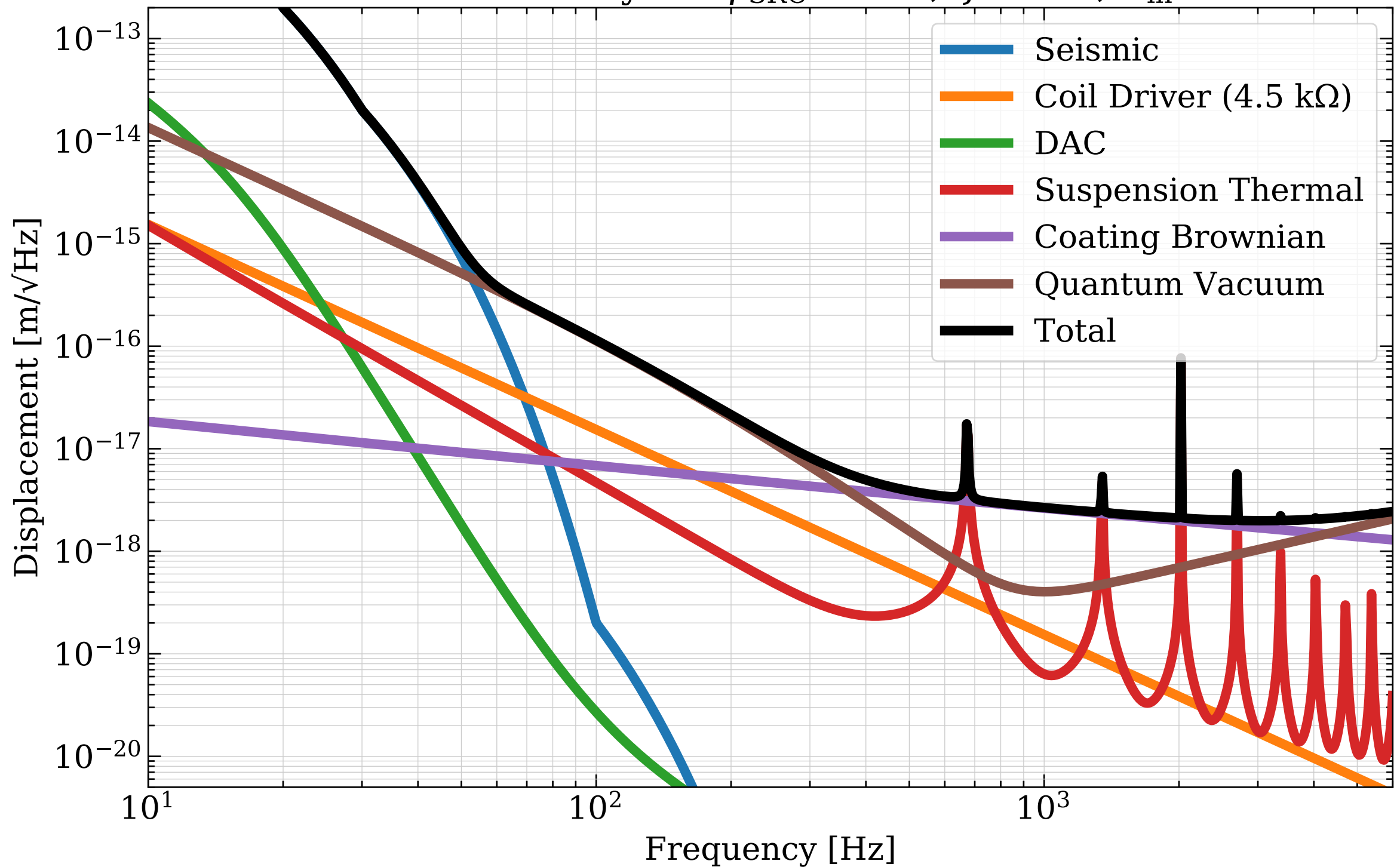
40m DARM sensitivity for \phi_{\text{SRC}} = 0.0^\circ , \zeta = 0.0^\circ , P_{\text{in}} = 20 \text{ W}
