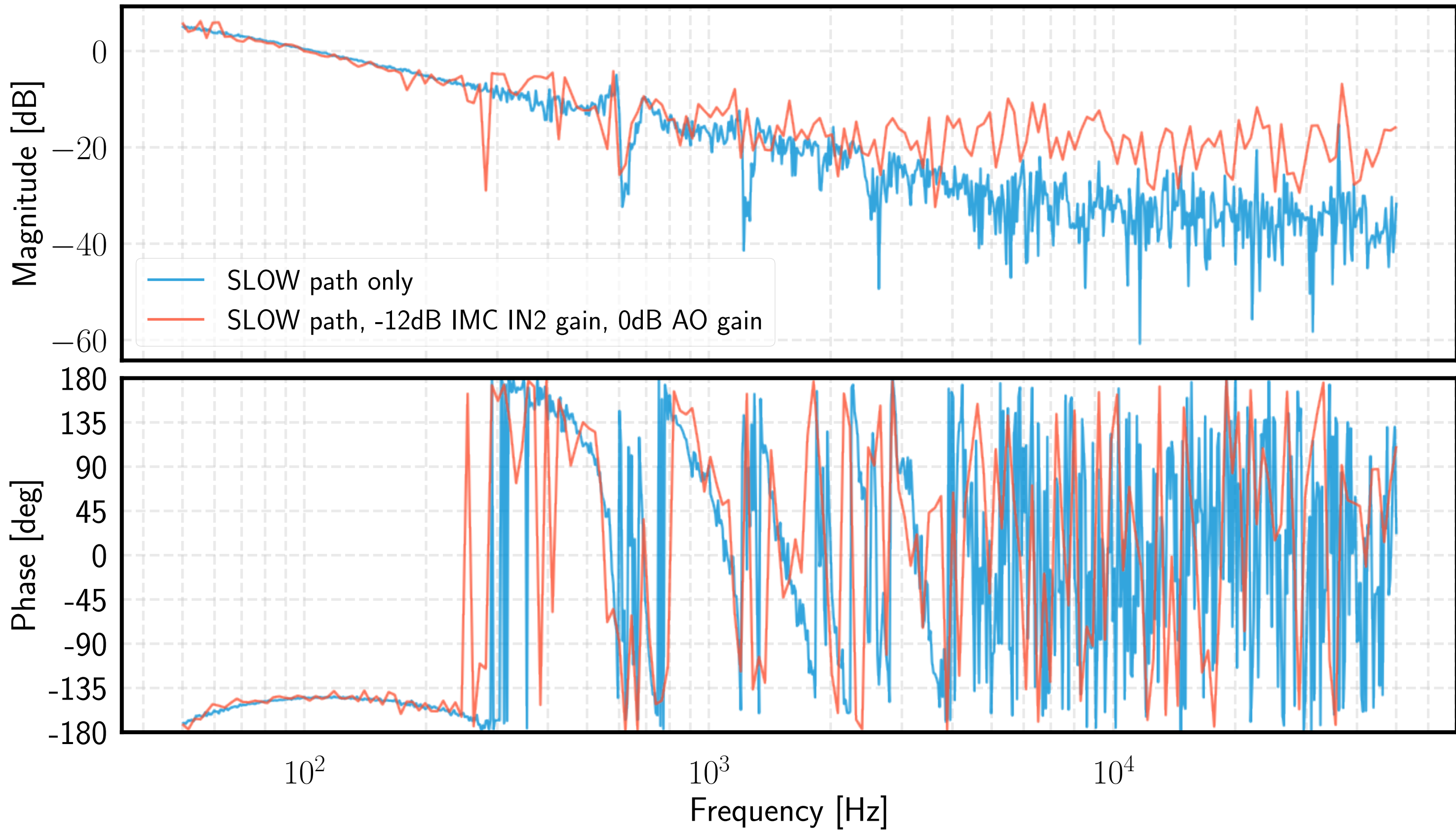
OLTF measurement for X arm length controlled by ALS beat through CM board
