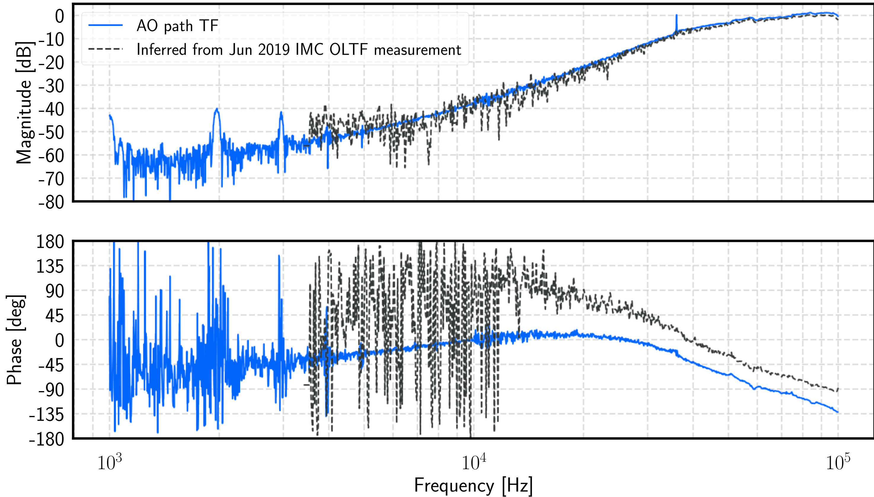
AO path TF, measured from TP2B on CM board to IMC TP1A
