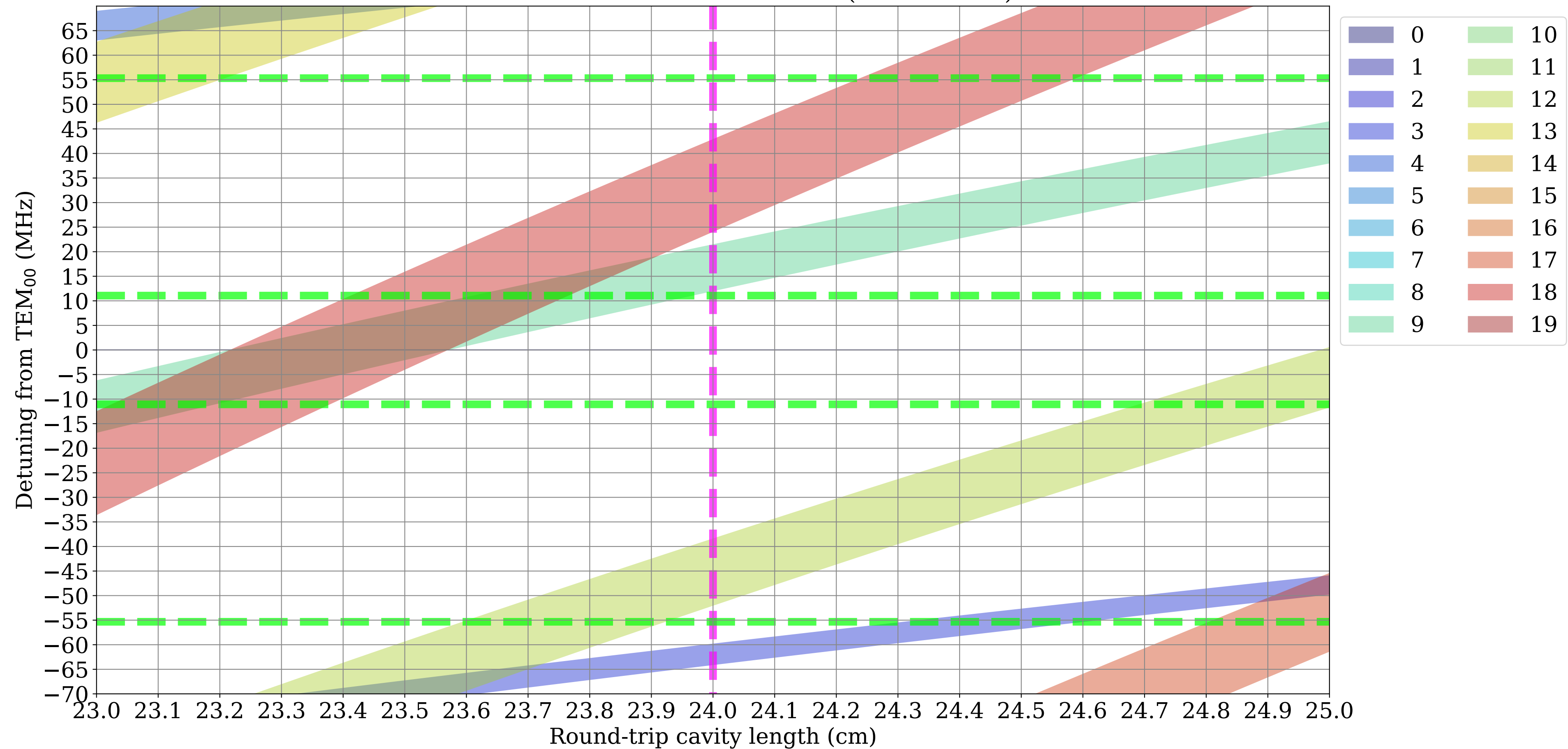
Locations of first 20 transverse modes (even and odd)
