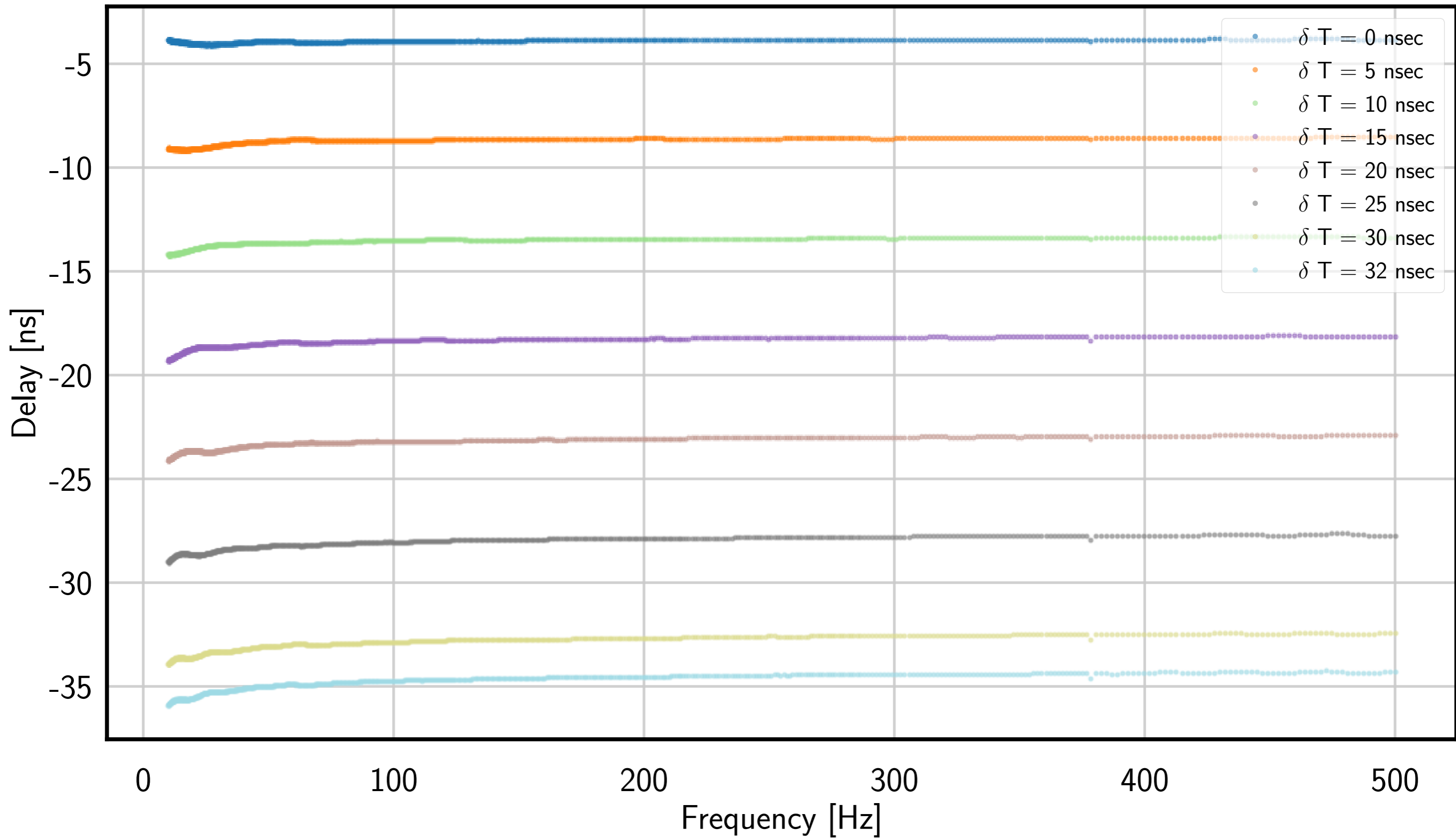
D050399 Delay line phase shifter effective frequency-dependent delay
