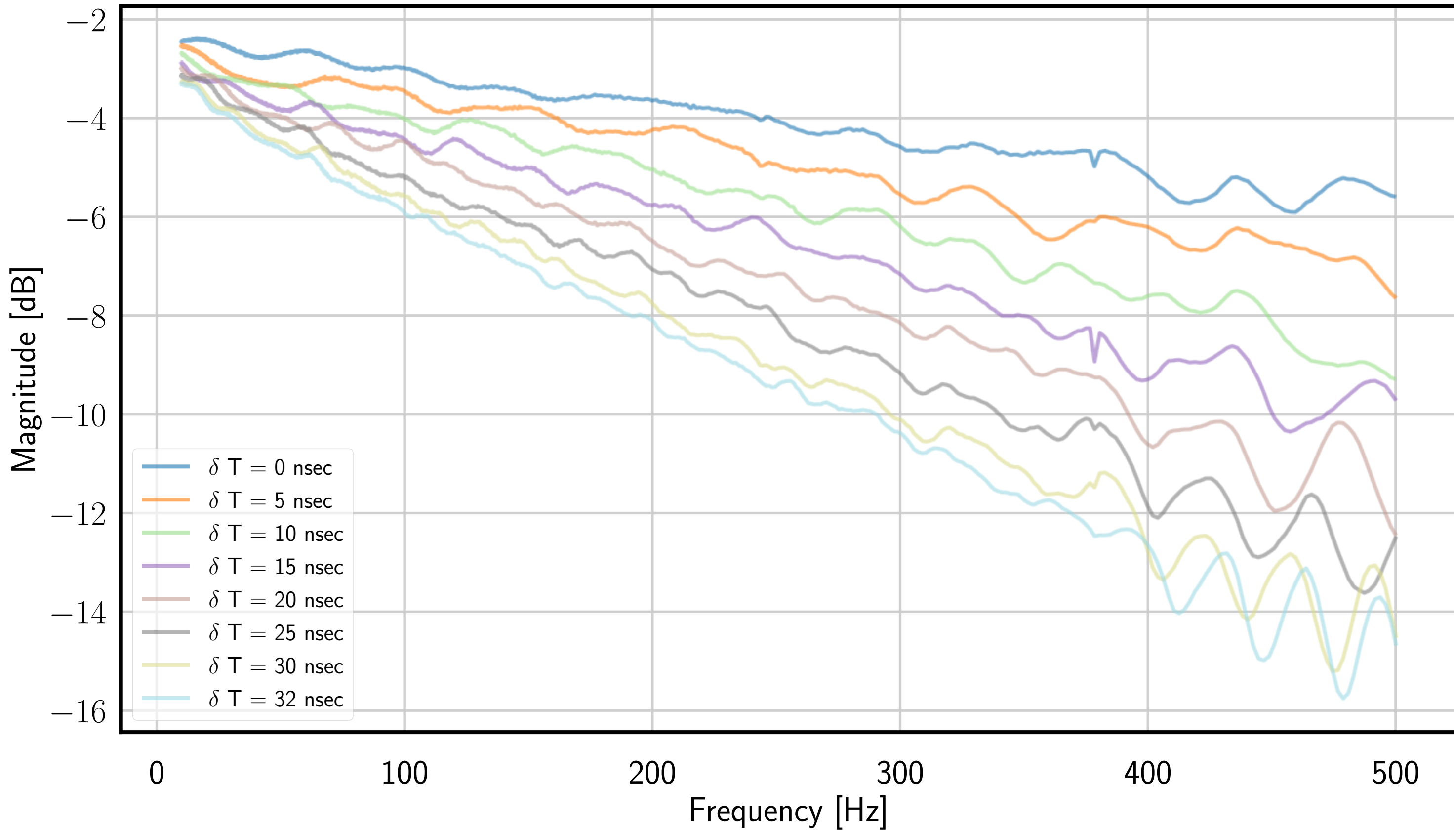
D050399 Delay line phase shifter insertion loss as a function of delay
