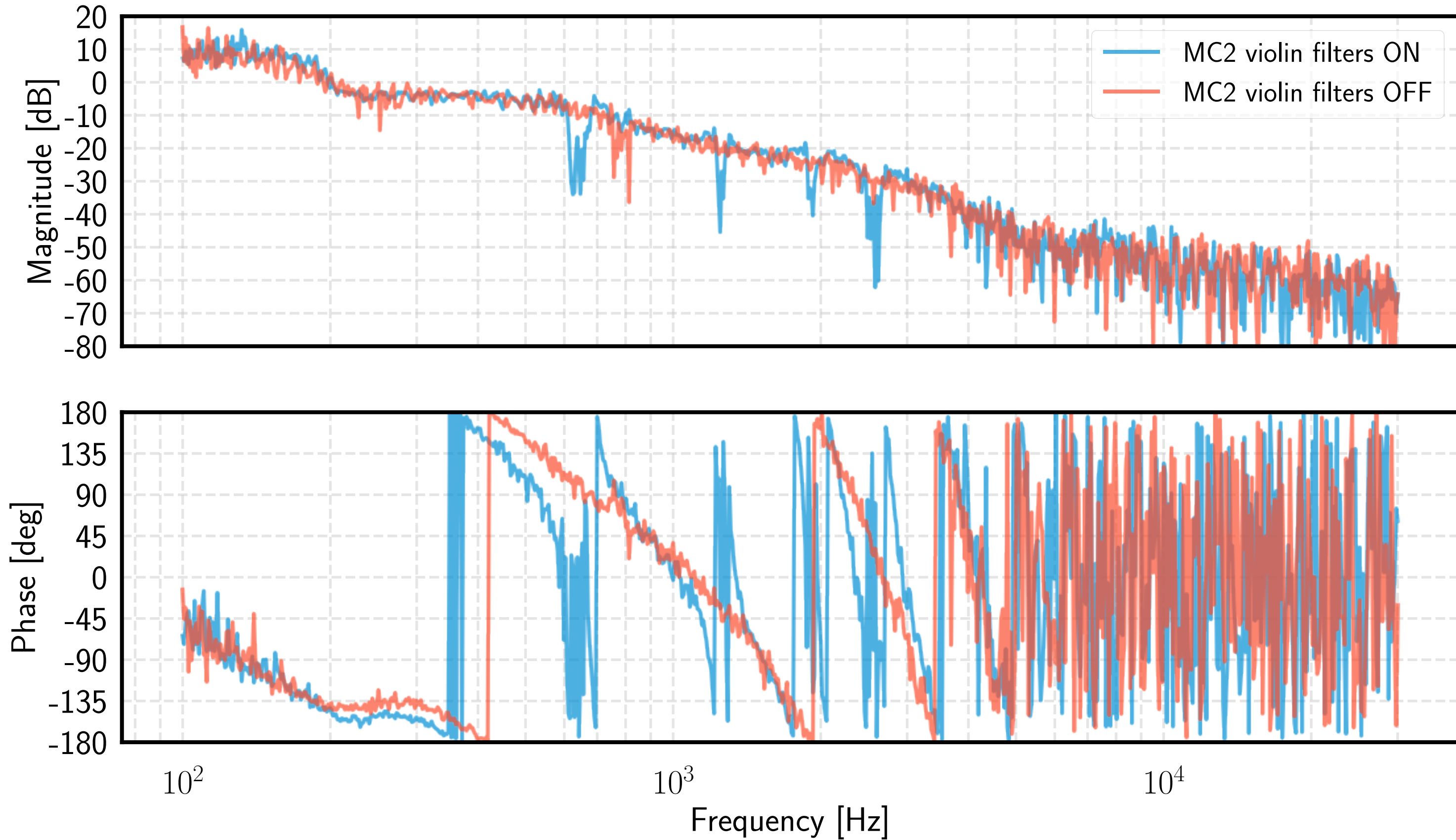
CARM OLTF with ALS and CM SLOW paths engaged, AO path disabled
