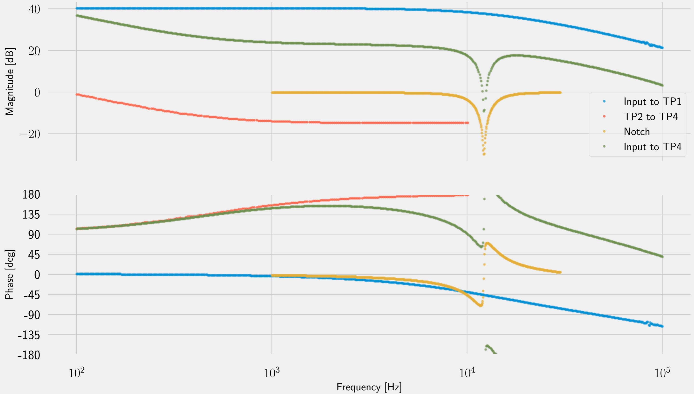
PMC Servo electronic TFs (VGA gain = 10dB)
