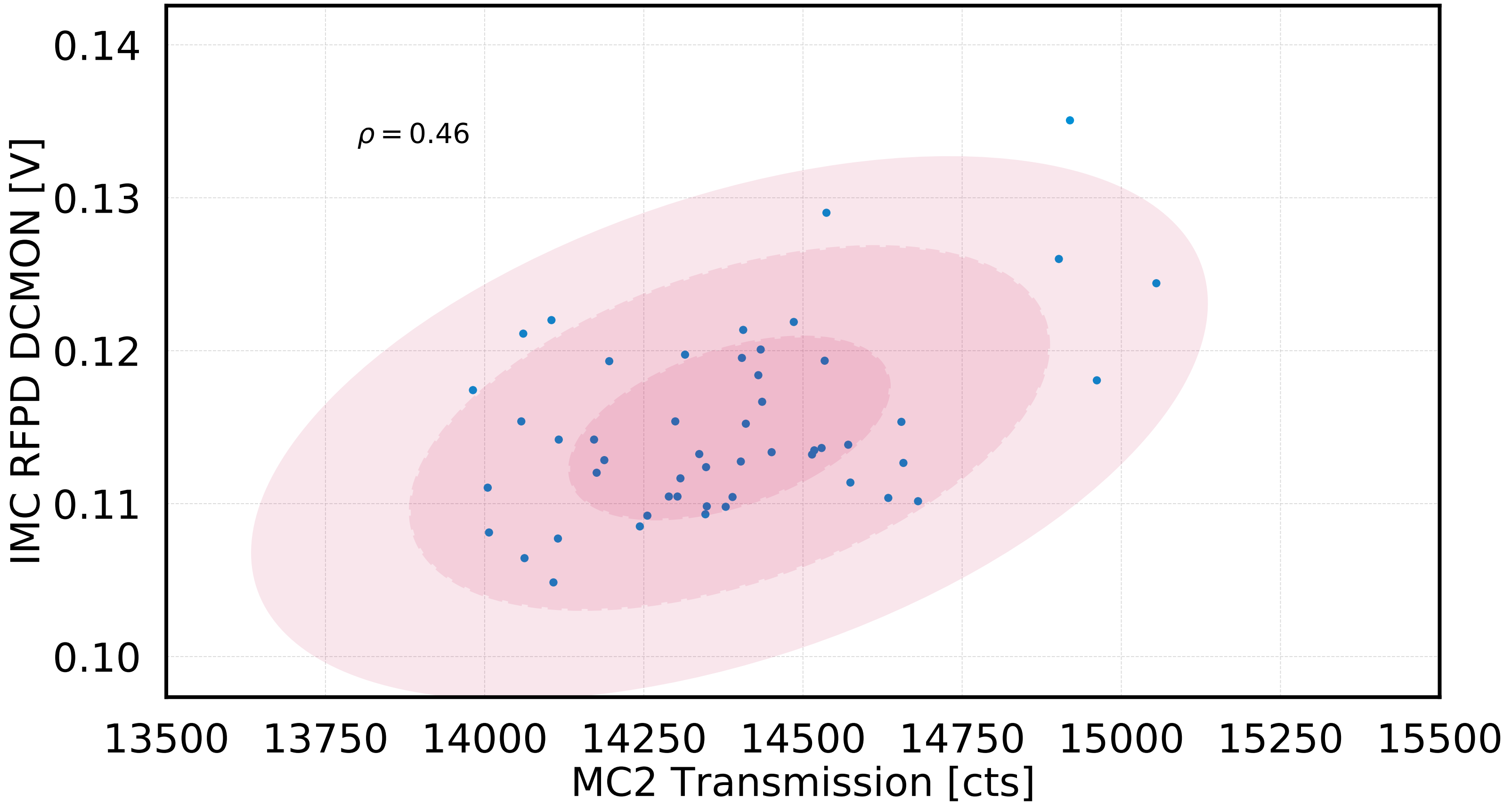
Correlation between MC2 Trans and IMC REFL DCMON
