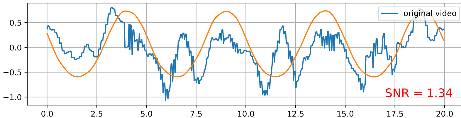
centroid from weighted sum
