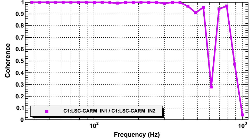
CARM Coherence function
