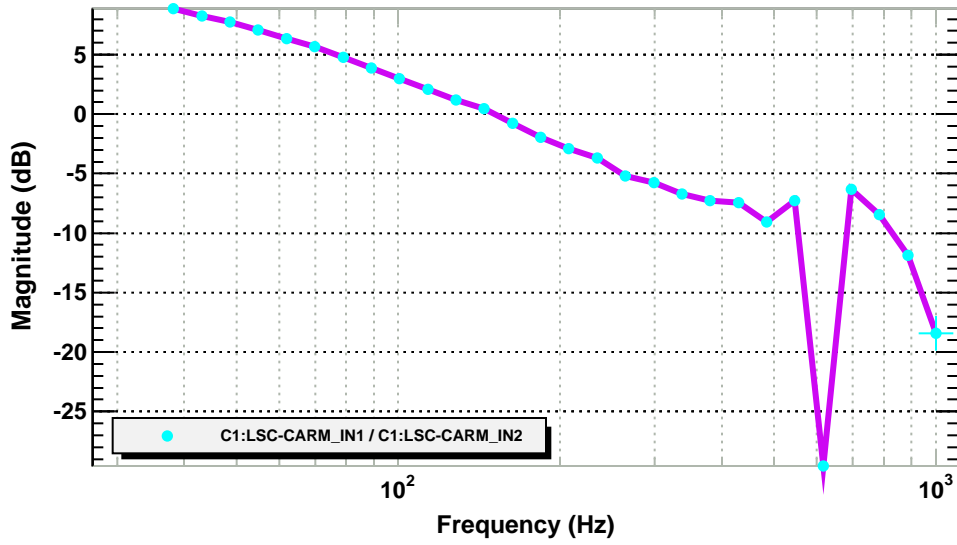
CARM Open Loop Gain
