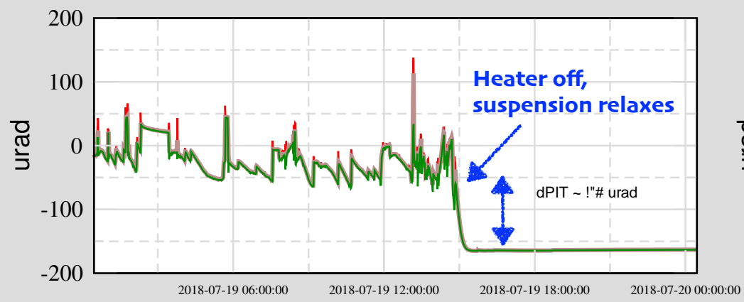
Ch 1: C1:SUS-ETMY_SUSPIT_INMON
