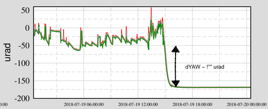
Ch 5: C1:SUS-ETMY_SUSYAW_INMON
