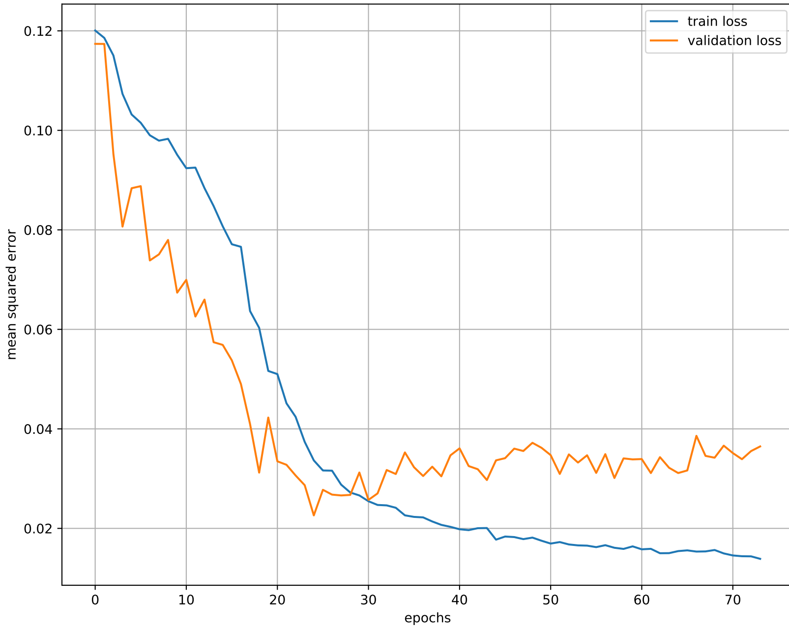
Learning_curves_replotted
