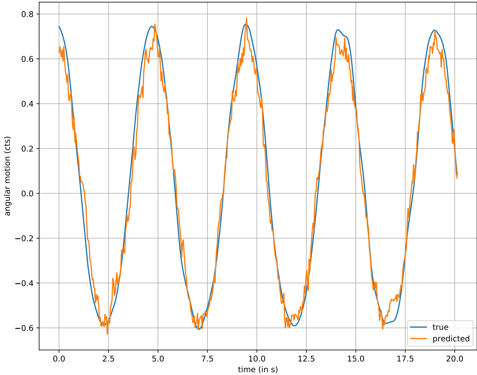
yaw_motion_test
