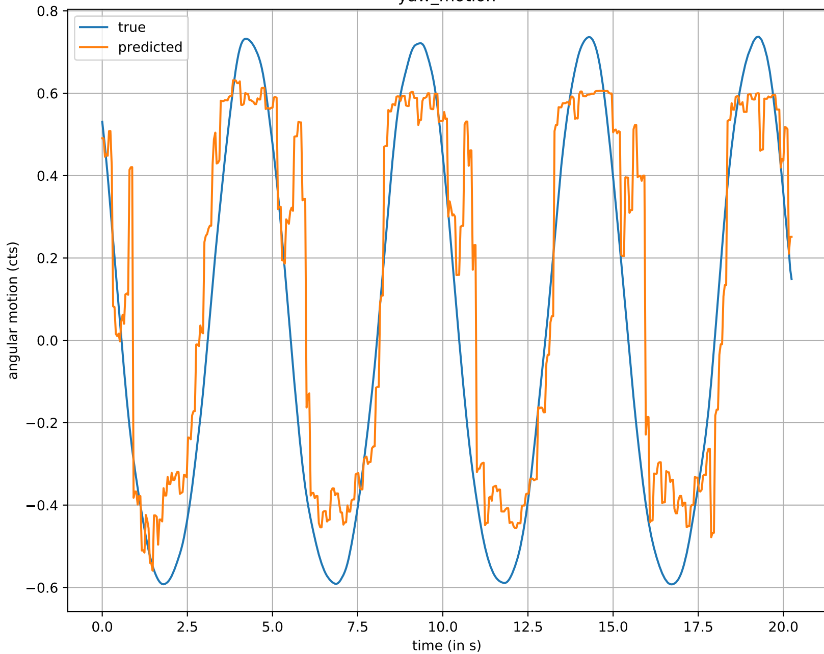
yaw_motion
