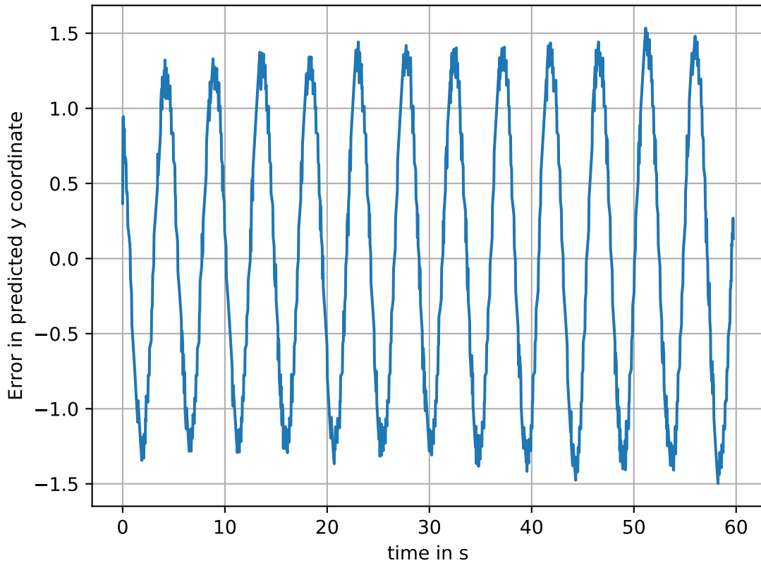
Error in prediction, normalised
