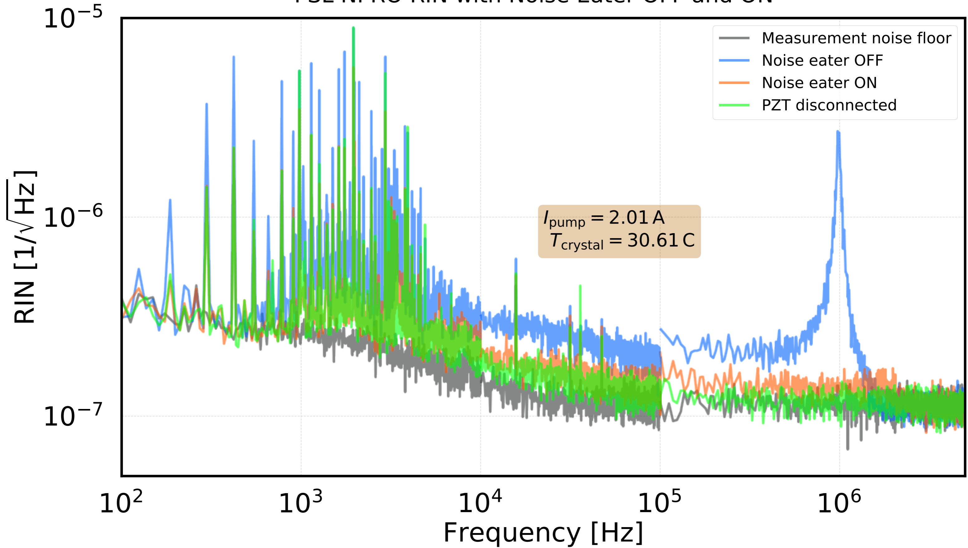
PSL NPRO RIN with Noise Eater OFF and ON
