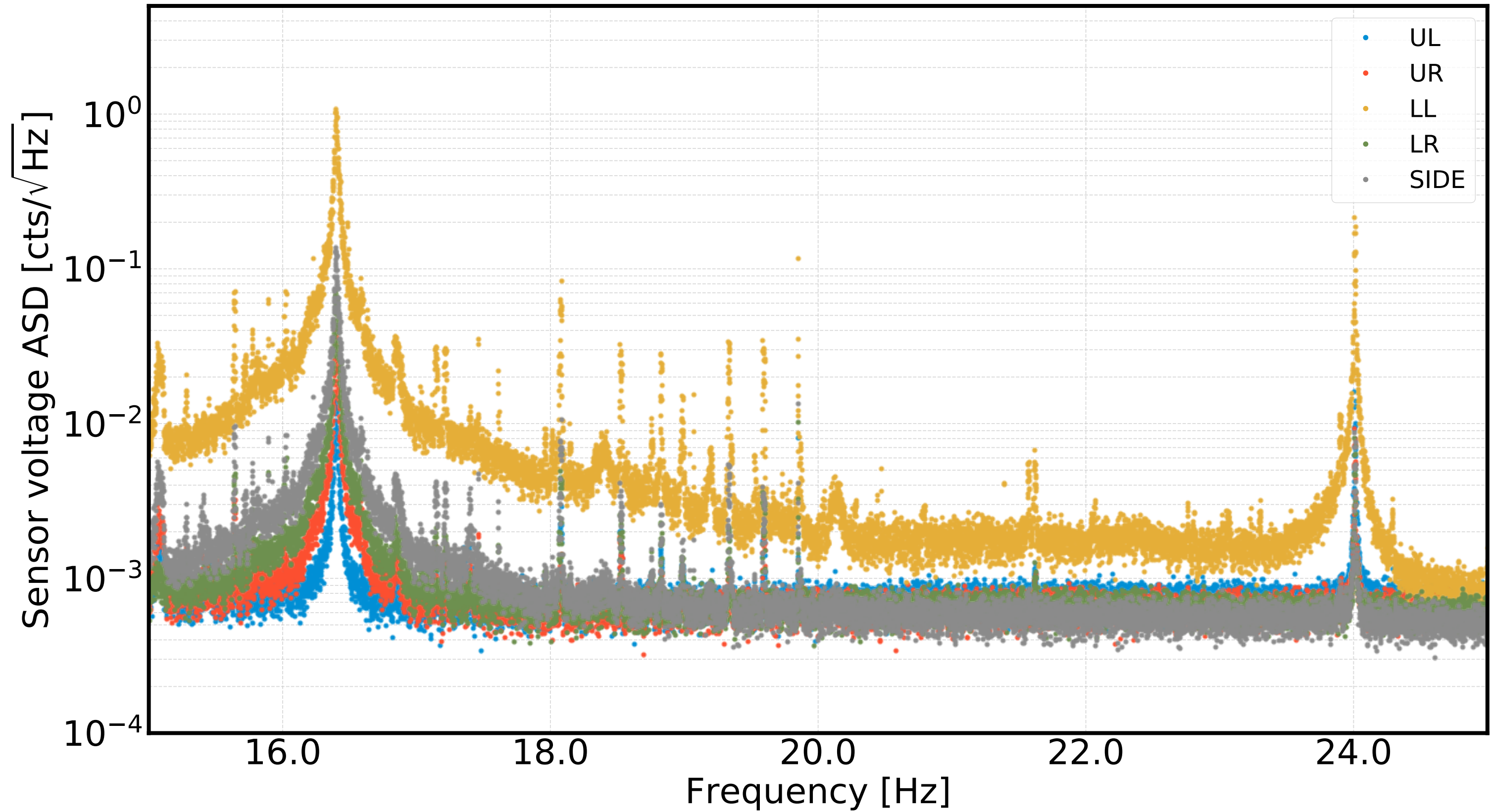
ETMY Sensor voltage spectra from 18 Apr 2019 2325 PDT for 10000 seconds
