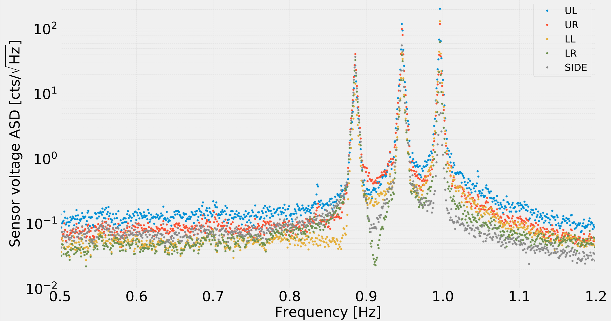
ETMY Sensor voltage spectra from 18 Apr 2019 2325 PDT for 10000 seconds
