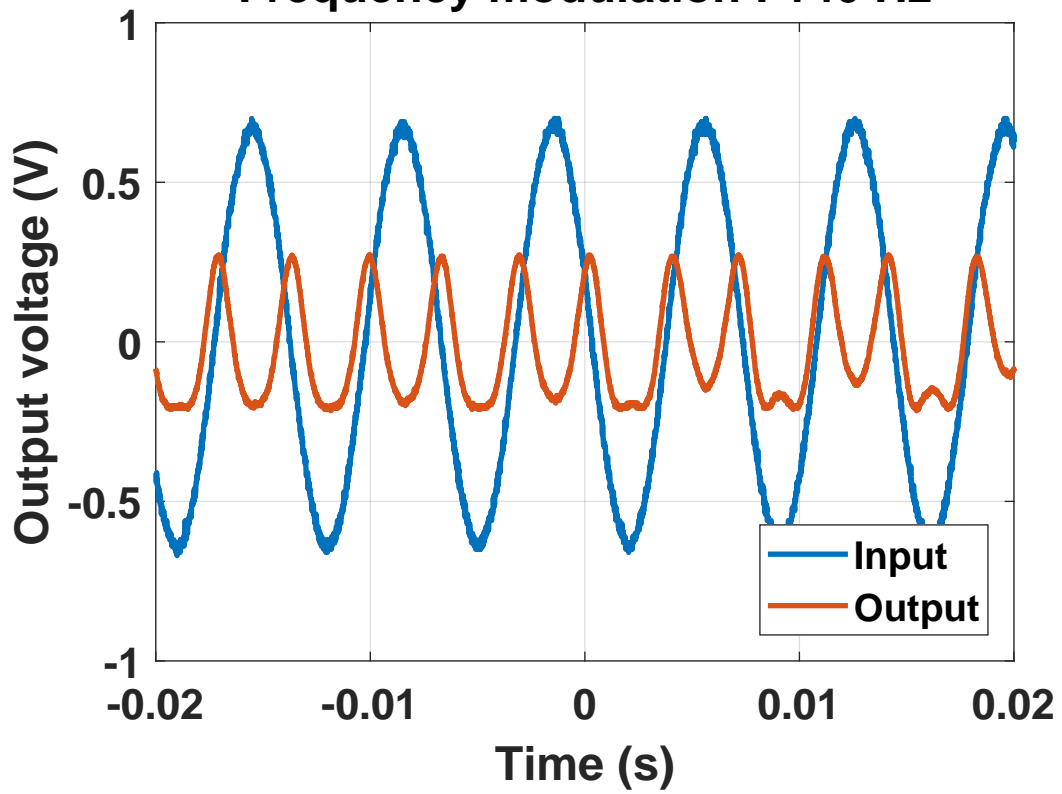
Frequency modulation : 140 Hz
