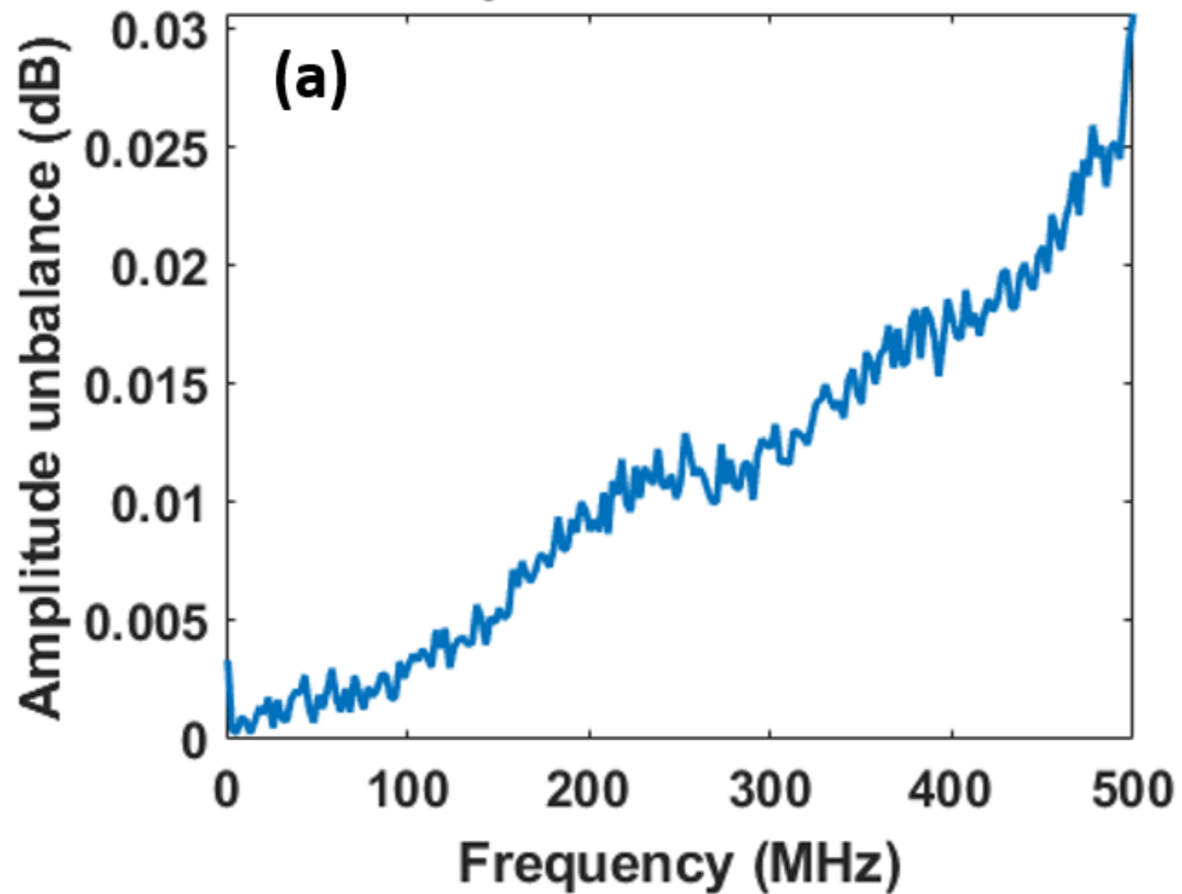
Amplitude unbalance
