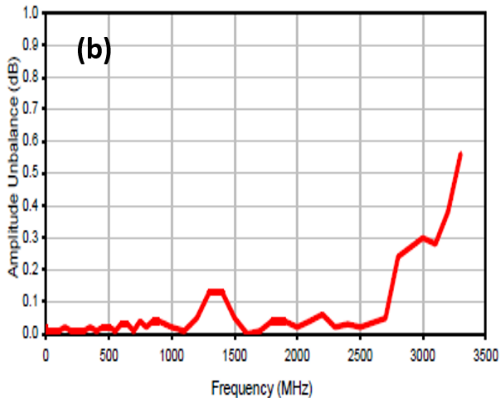
Amplitude Unbalance
