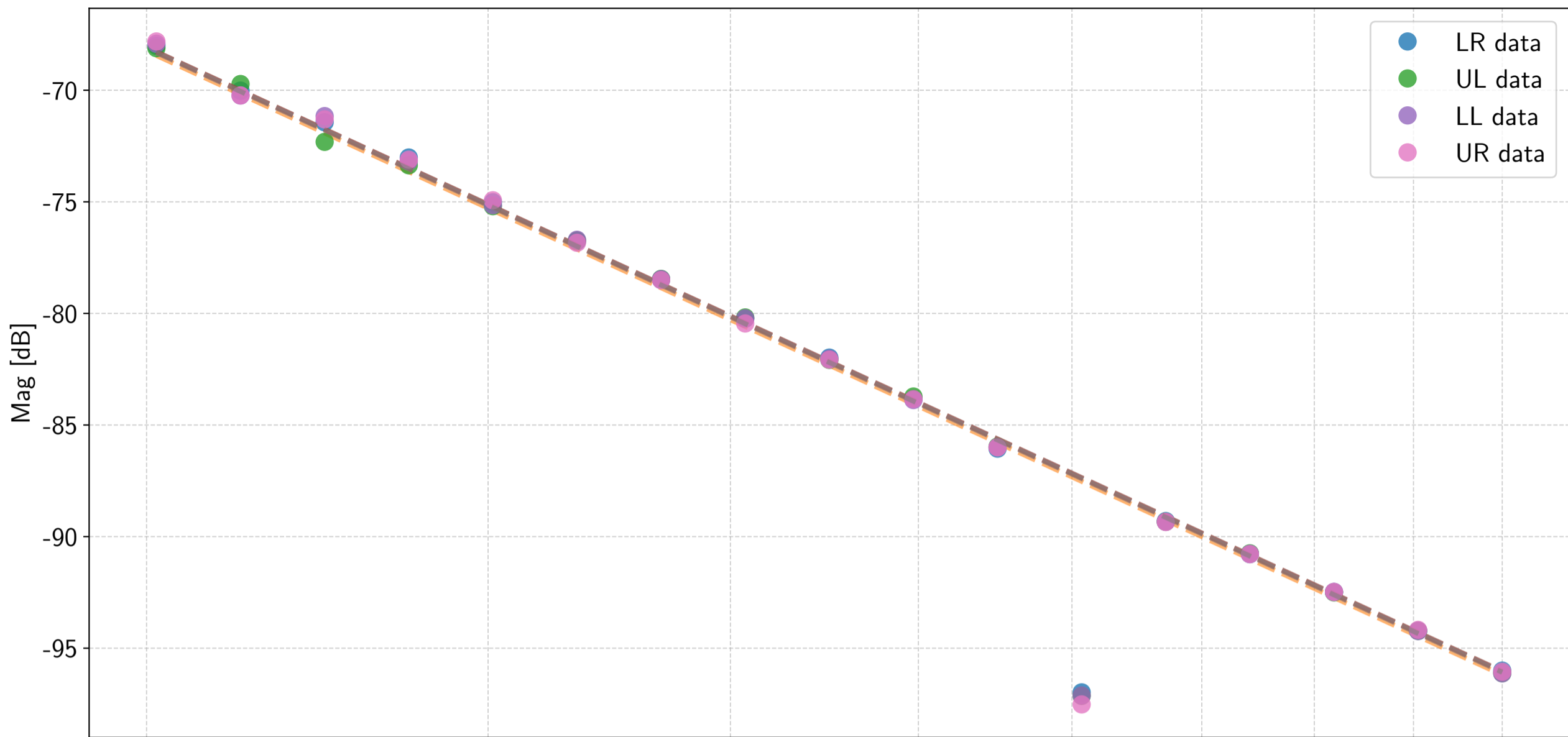
ETMY relative coil actuation strength witnessed by OL PIT
