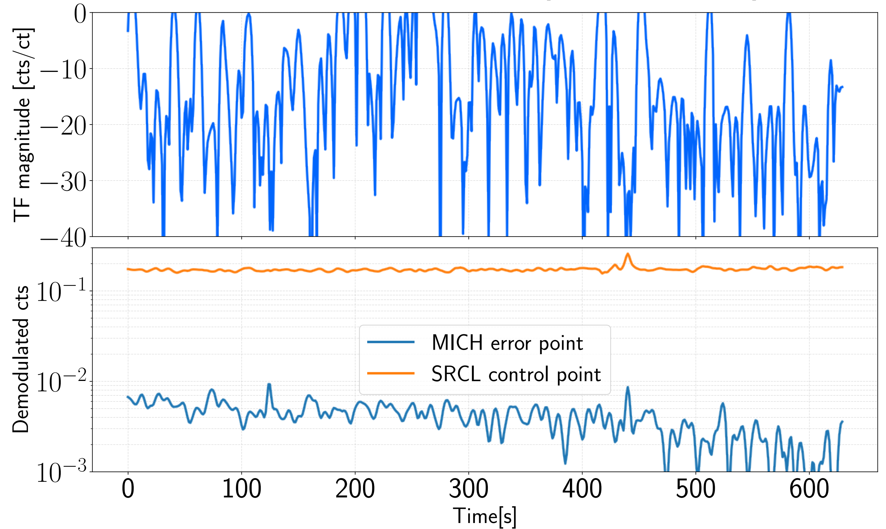
Time variation of SRCL coupling to MICH [0.1 Hz LPF post-mixer]
