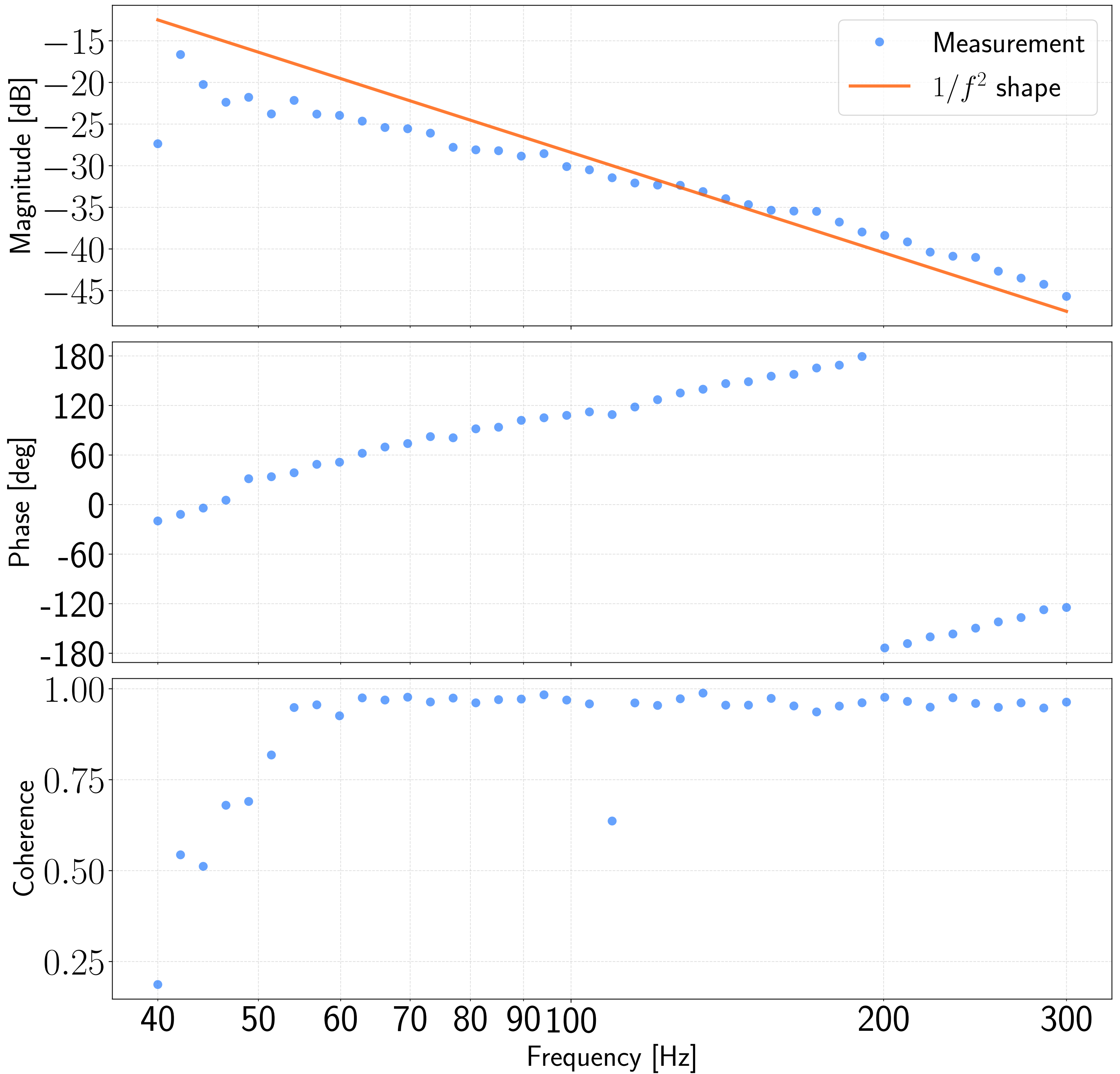
Swept-sine measurement of transfer function from SRCL OUT to MICH IN
