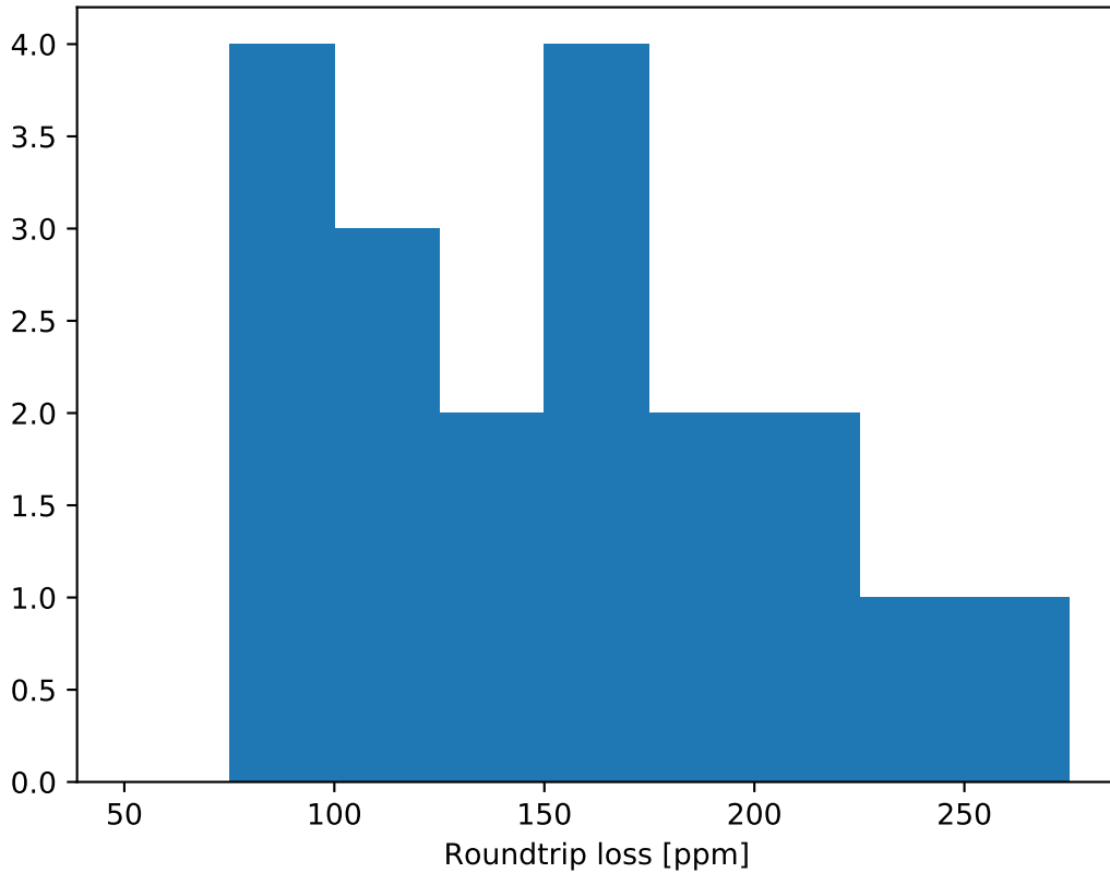
DCREFL AS-Port YARM Loss Histogram
